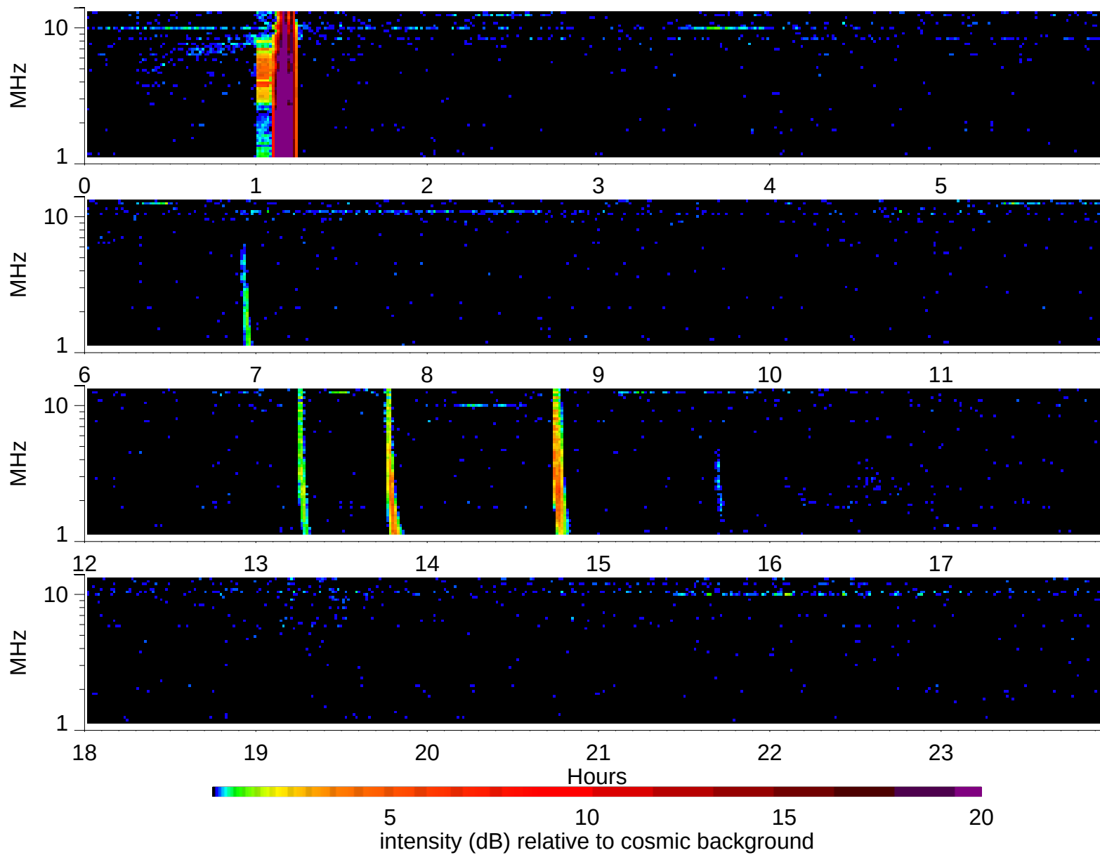
Wind Waves RAD2 receiver: 1998/2/9
