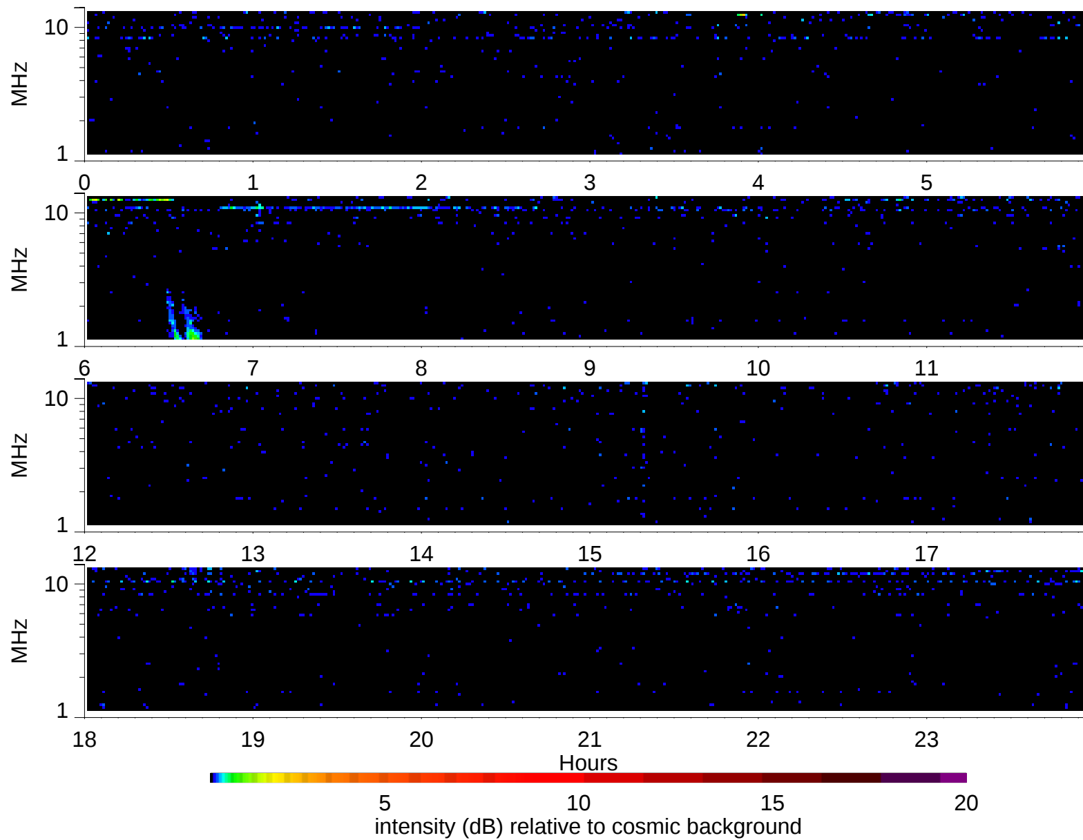
Wind Waves RAD2 receiver: 1998/2/10
