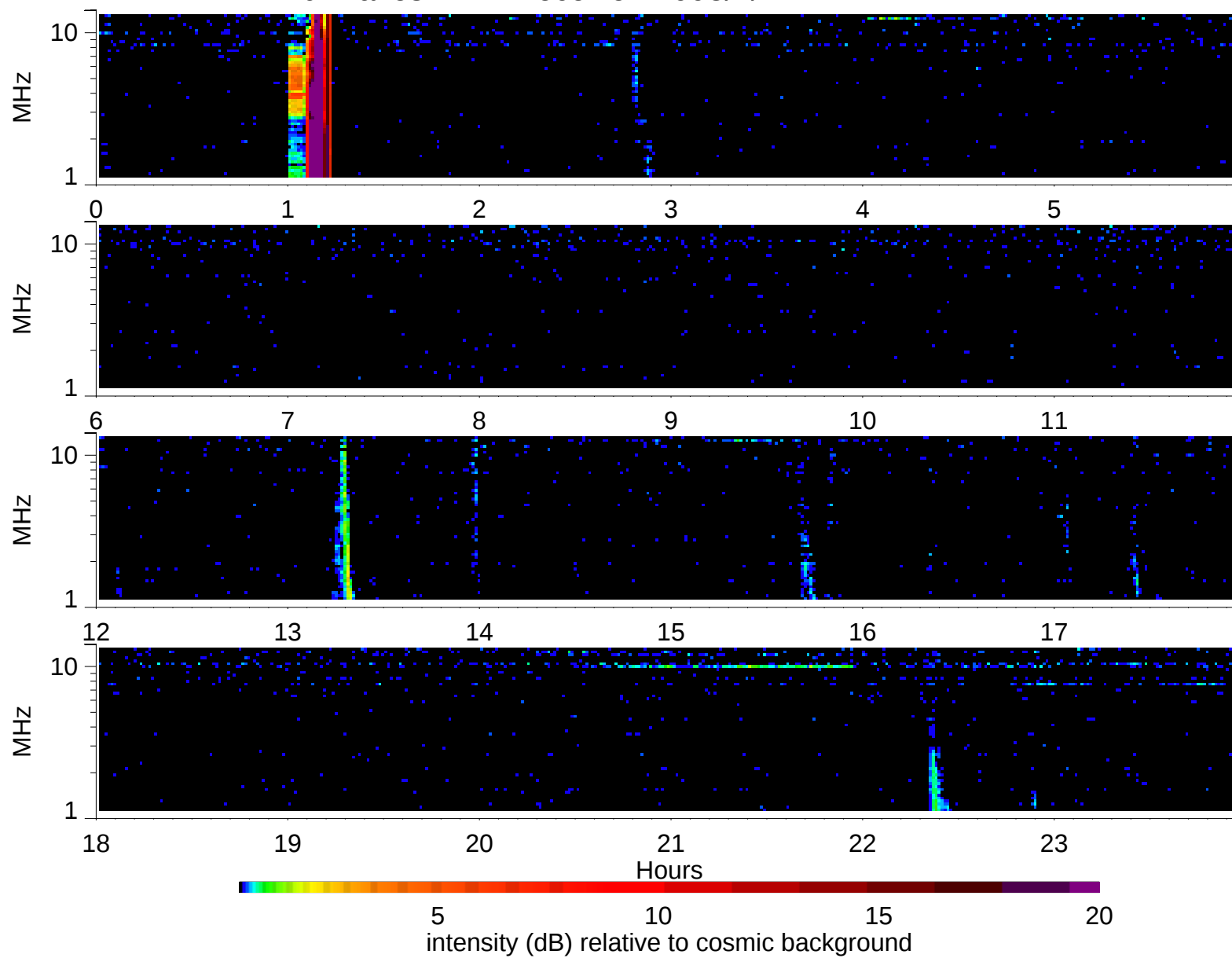
Wind Waves RAD2 receiver: 1998/2/11
