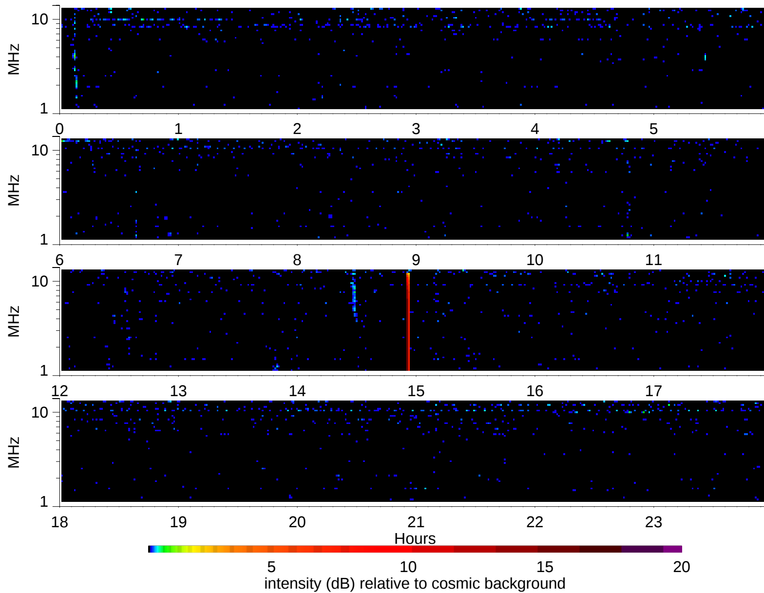
Wind Waves RAD2 receiver: 1998/2/12
