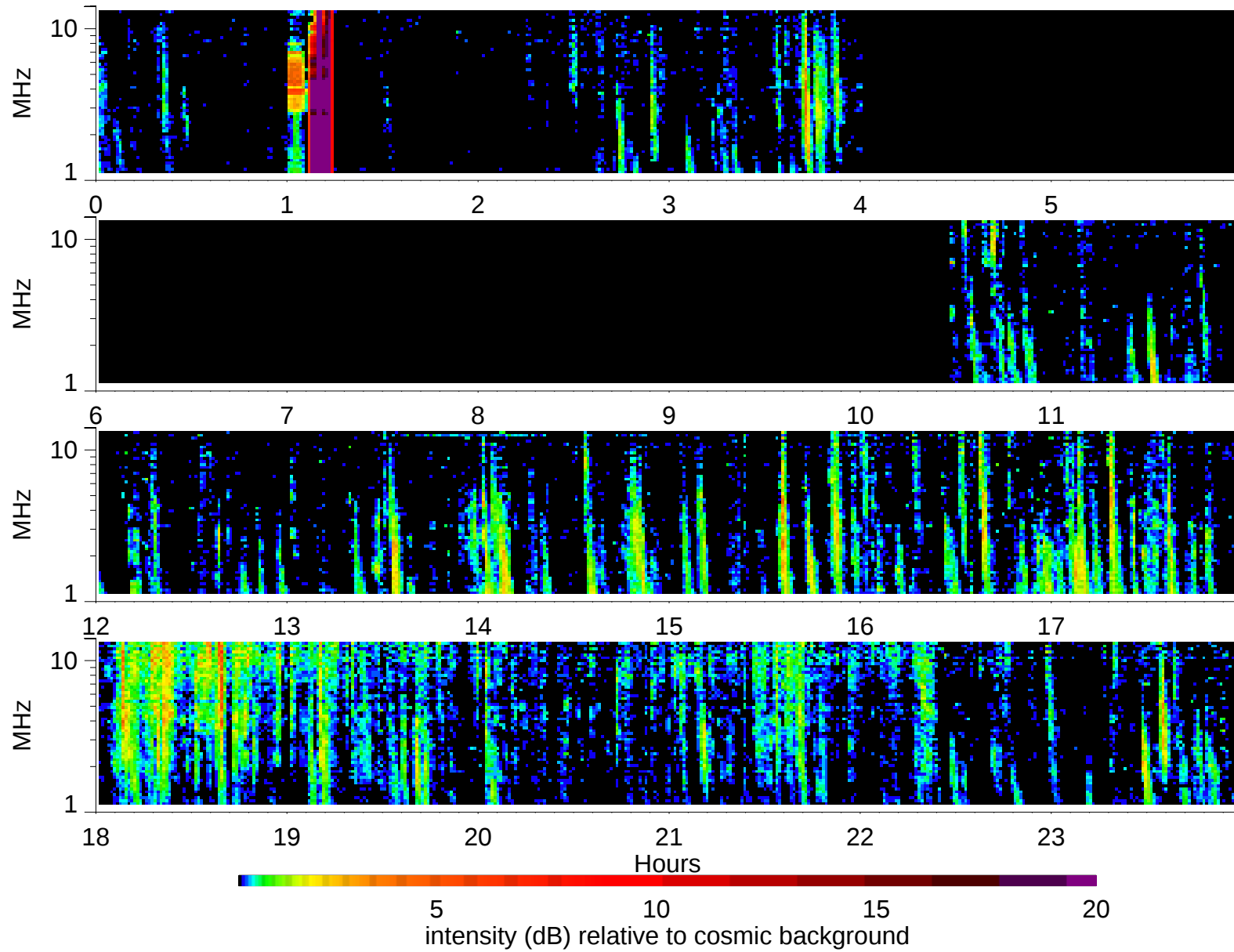
Wind Waves RAD2 receiver: 1998/2/15
