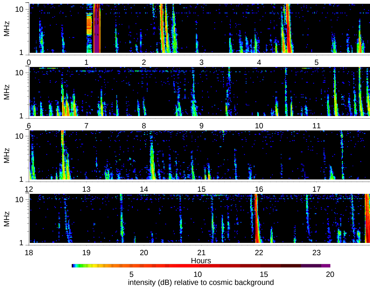
Wind Waves RAD2 receiver: 1998/2/17
