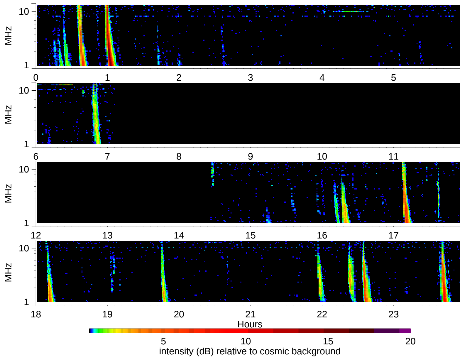
Wind Waves RAD2 receiver: 1998/2/20
