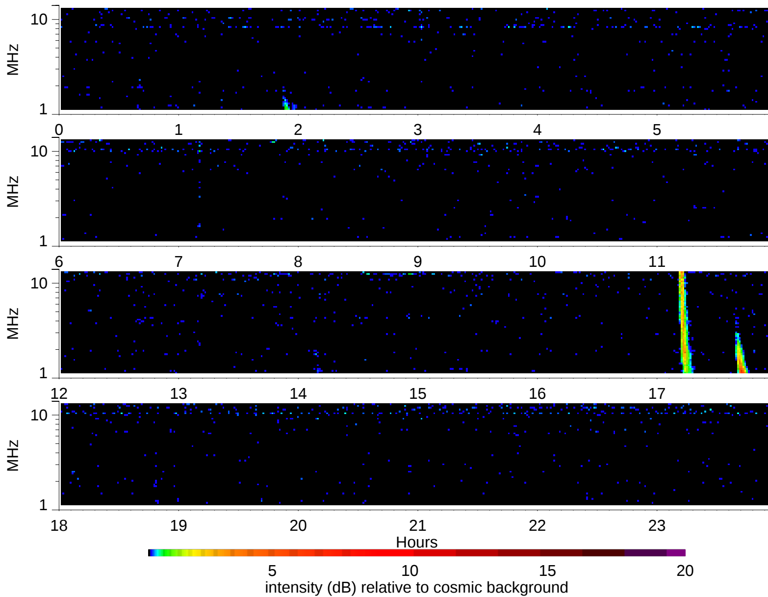
Wind Waves RAD2 receiver: 1998/2/24
