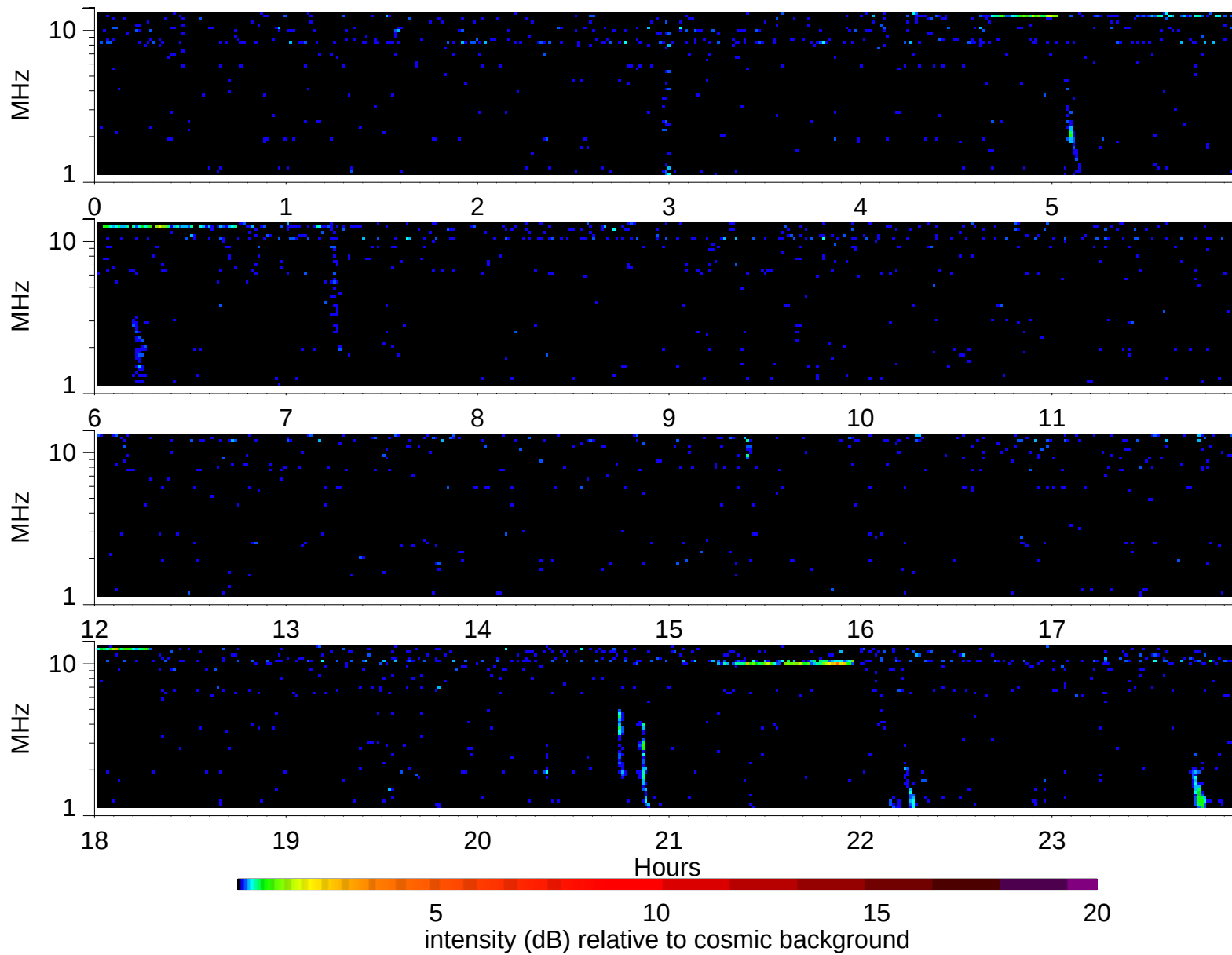
Wind Waves RAD2 receiver: 1998/3/2
