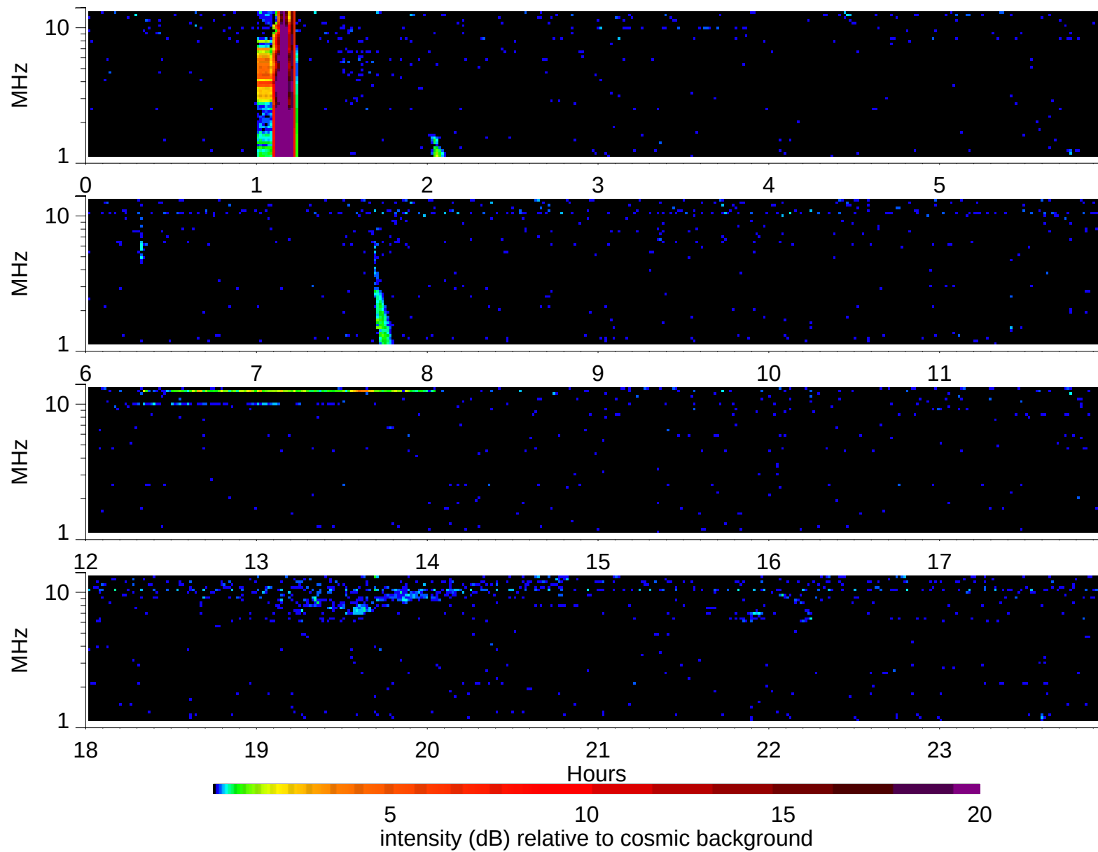
Wind Waves RAD2 receiver: 1998/3/5
