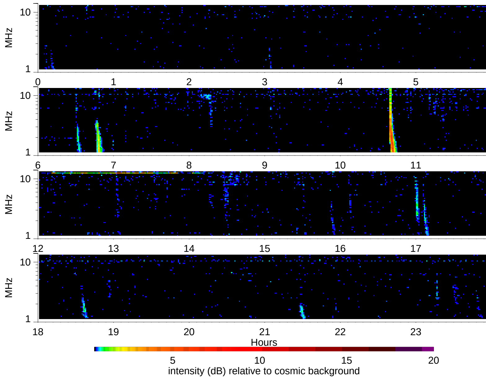
Wind Waves RAD2 receiver: 1998/3/6
