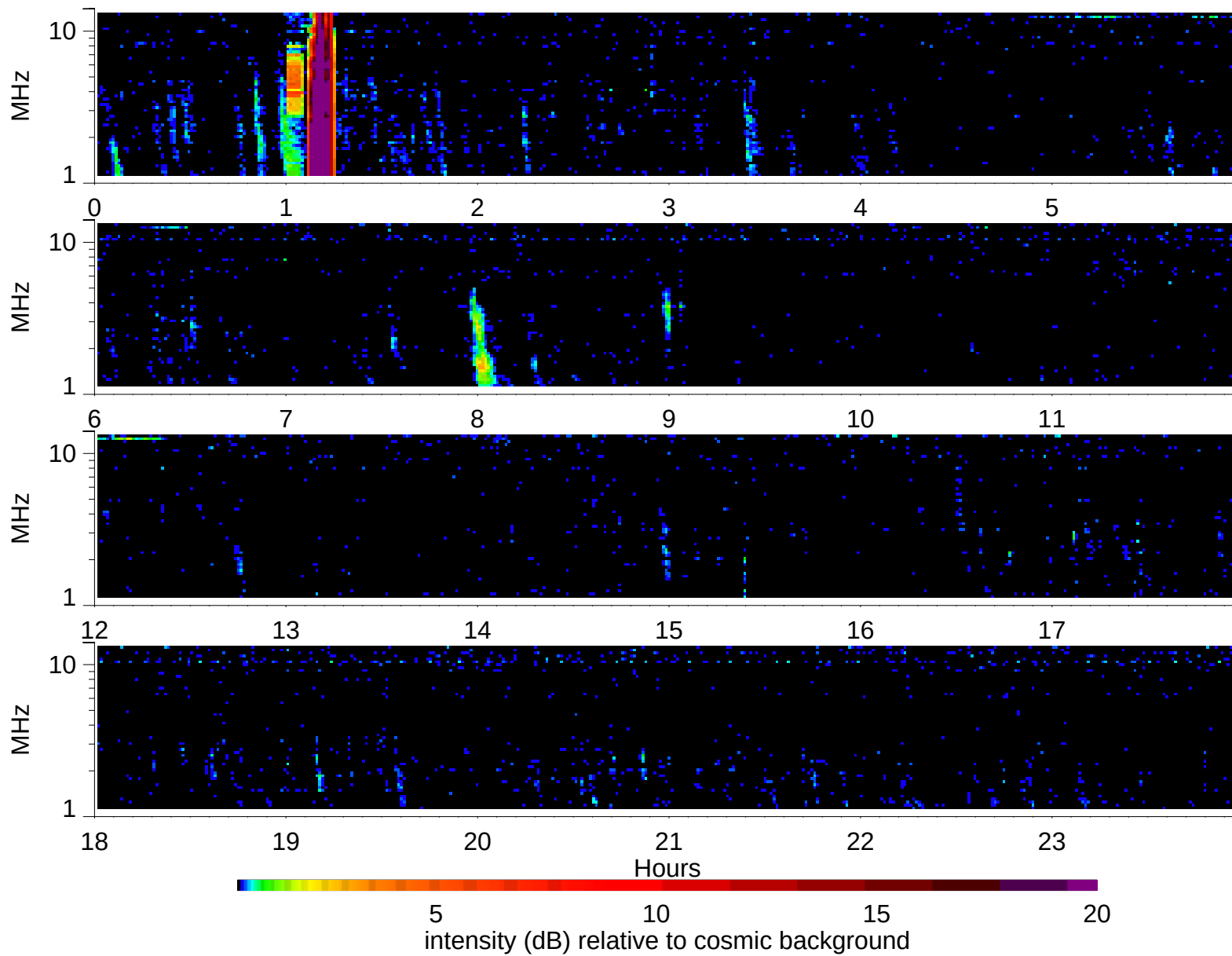
Wind Waves RAD2 receiver: 1998/3/7
