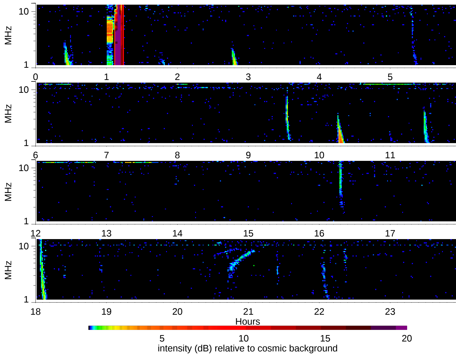
Wind Waves RAD2 receiver: 1998/3/9
