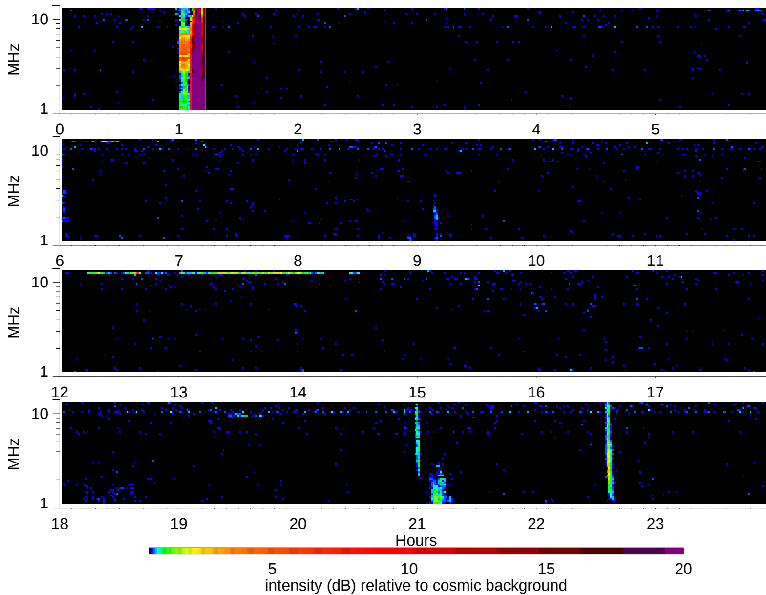
Wind Waves RAD2 receiver: 1998/3/13
