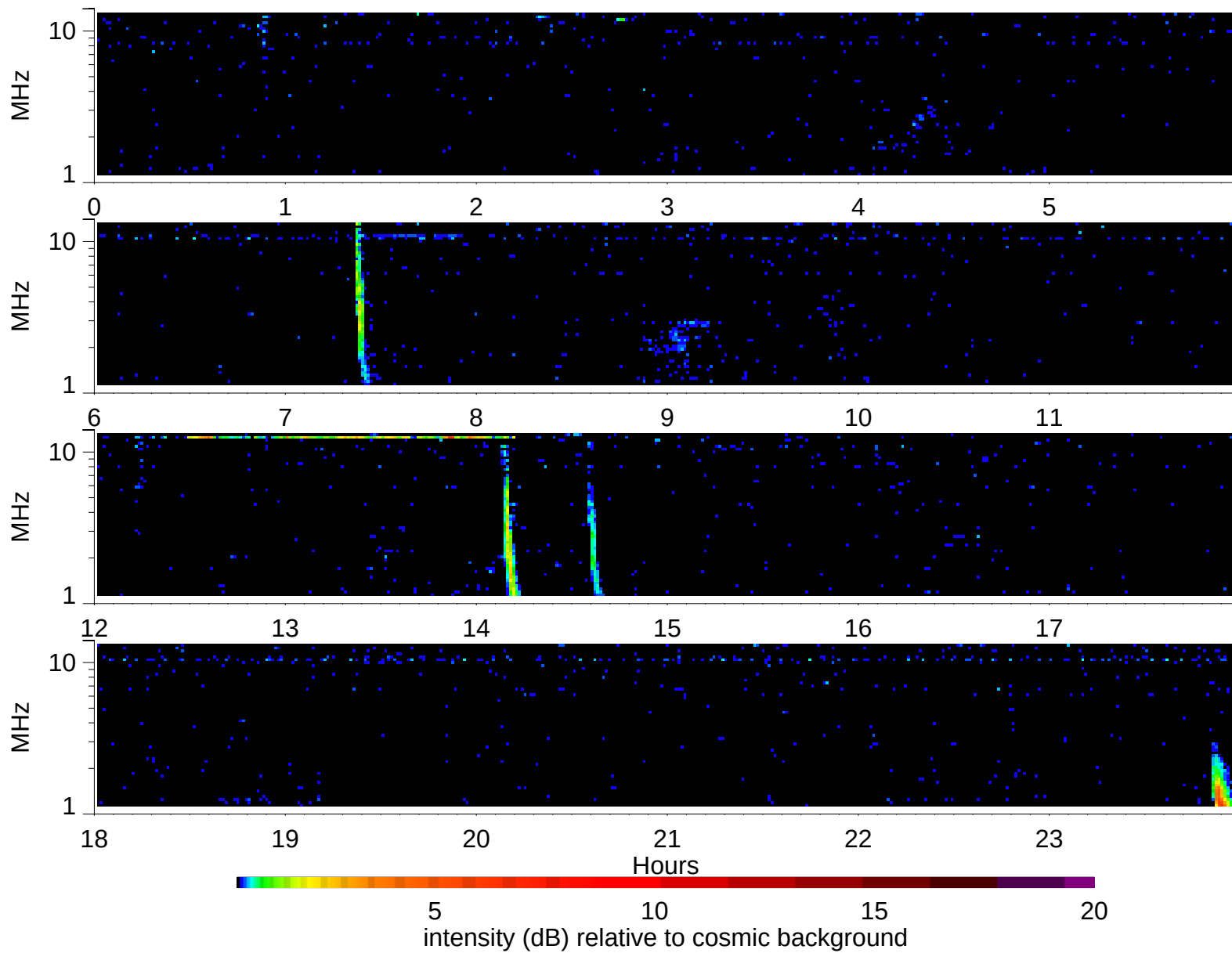
Wind Waves RAD2 receiver: 1998/3/14
