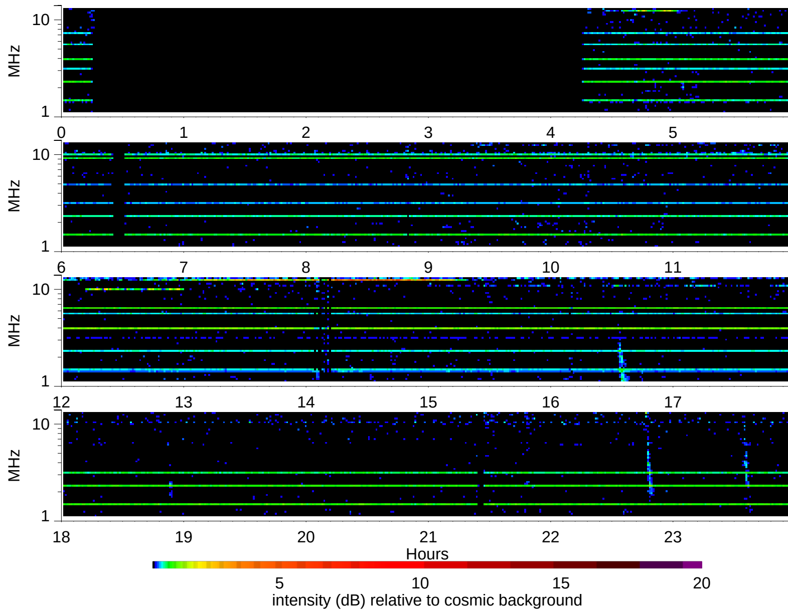
Wind Waves RAD2 receiver: 1998/3/15
