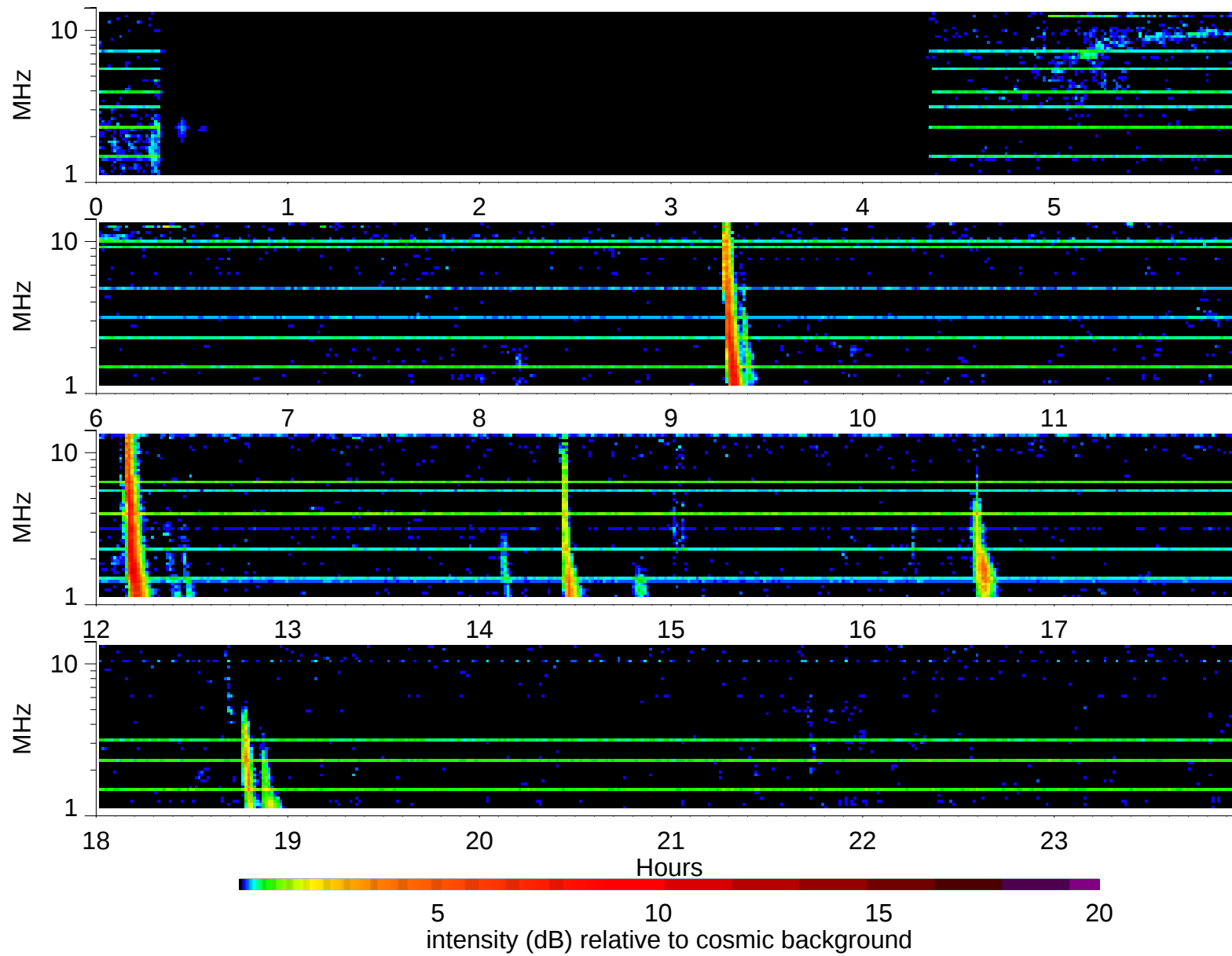
Wind Waves RAD2 receiver: 1998/3/18
