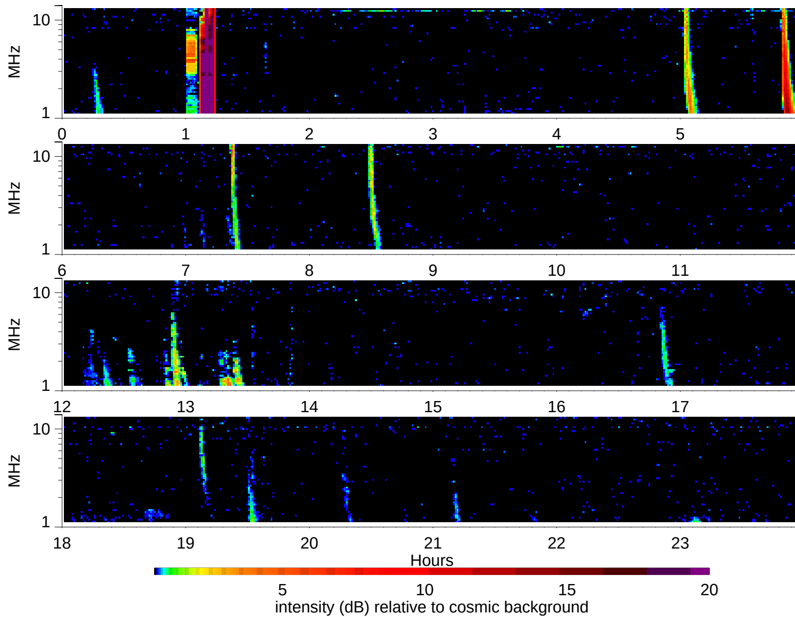
Wind Waves RAD2 receiver: 1998/3/25
