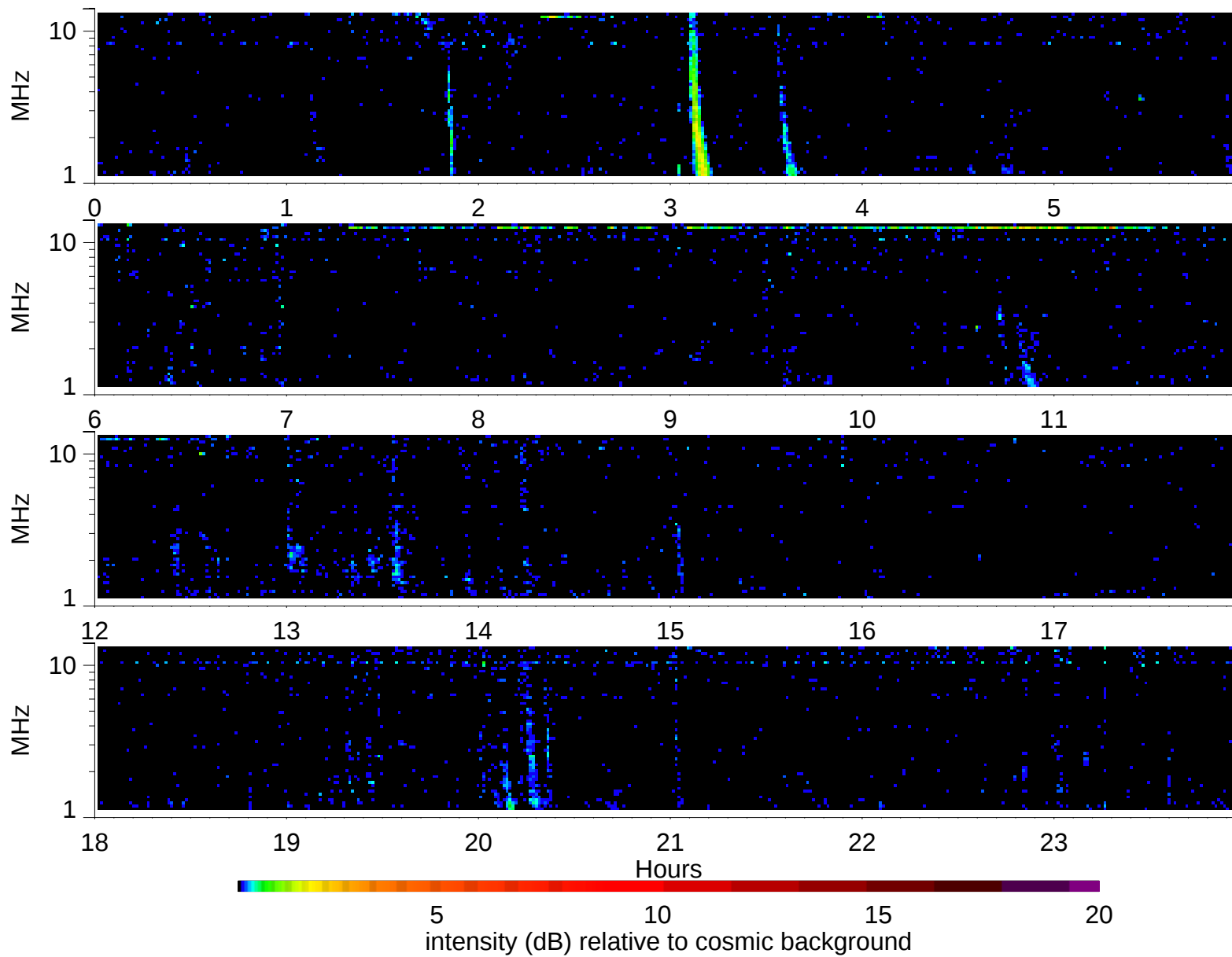
Wind Waves RAD2 receiver: 1998/3/26
