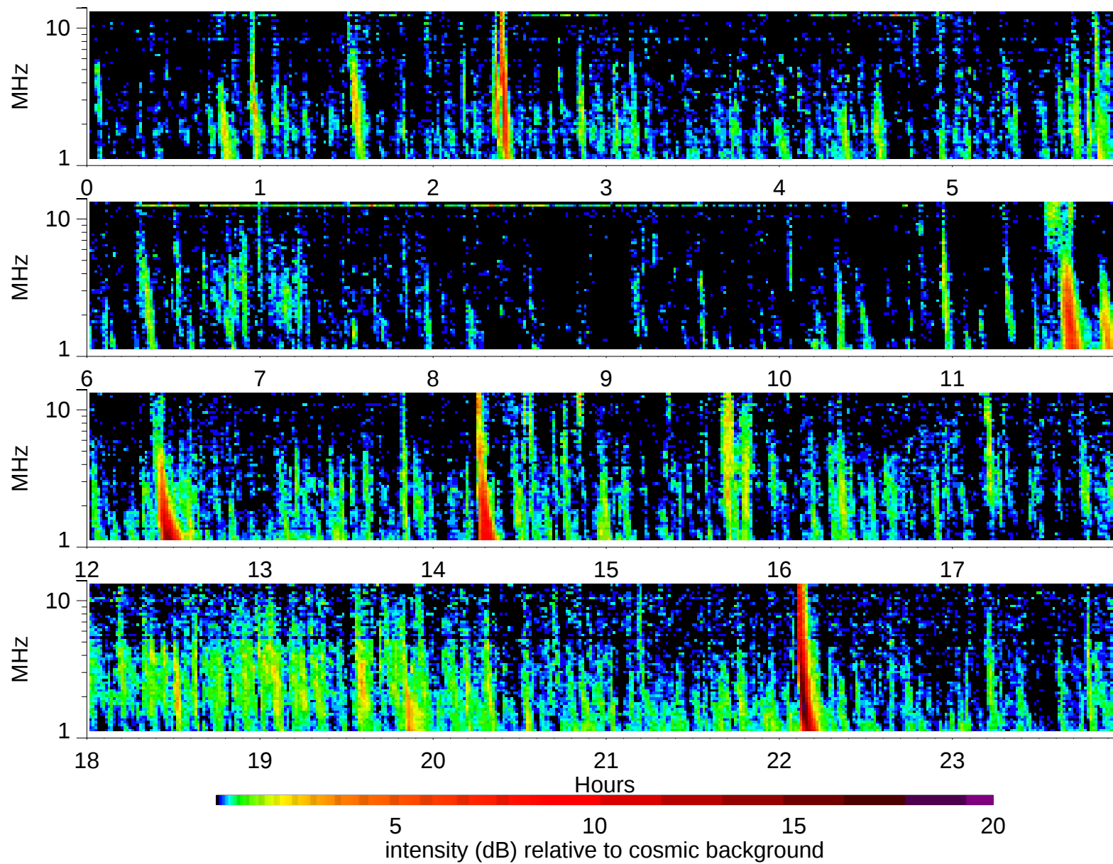
Wind Waves RAD2 receiver: 1998/4/1
