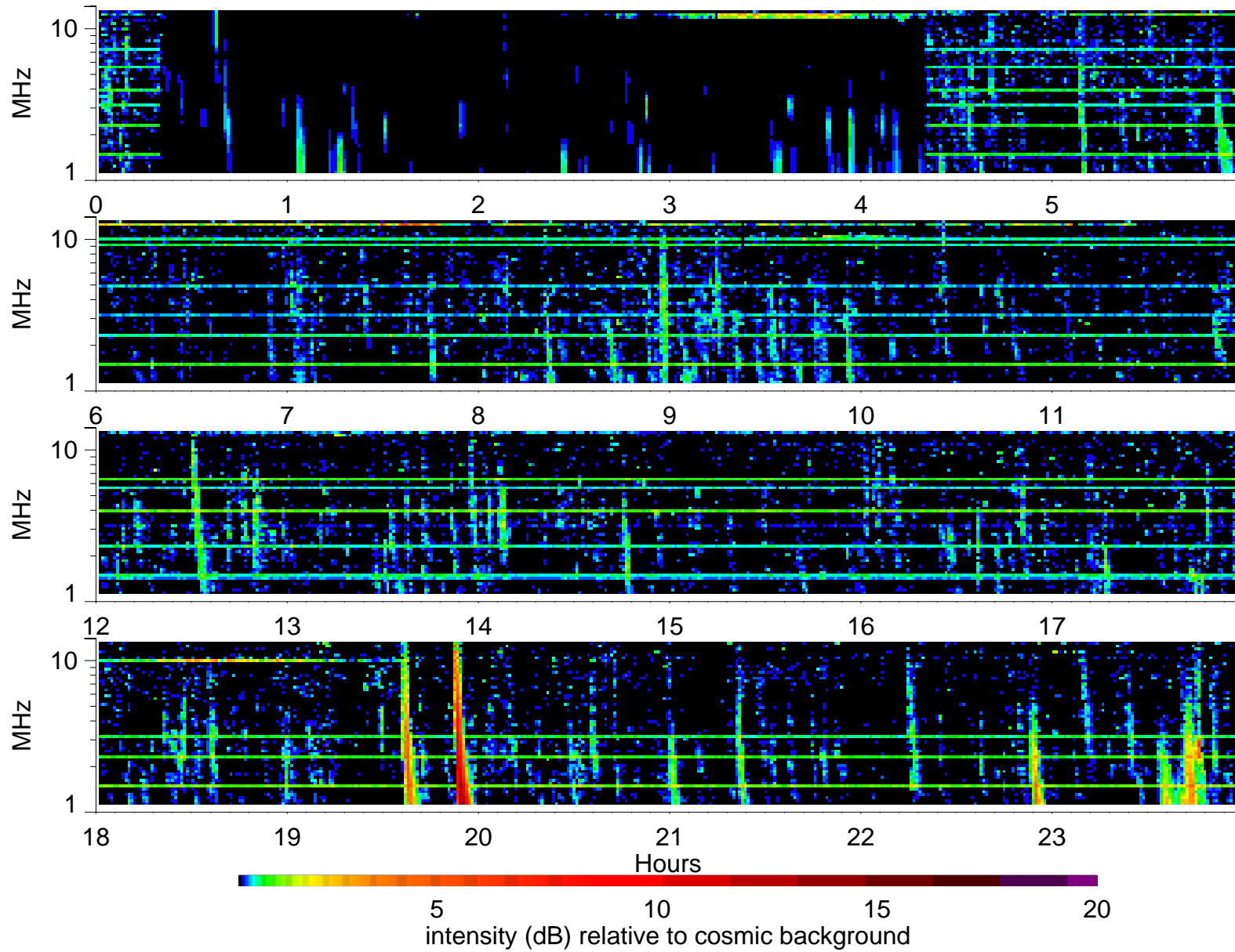
Wind Waves RAD2 receiver: 1998/4/3
