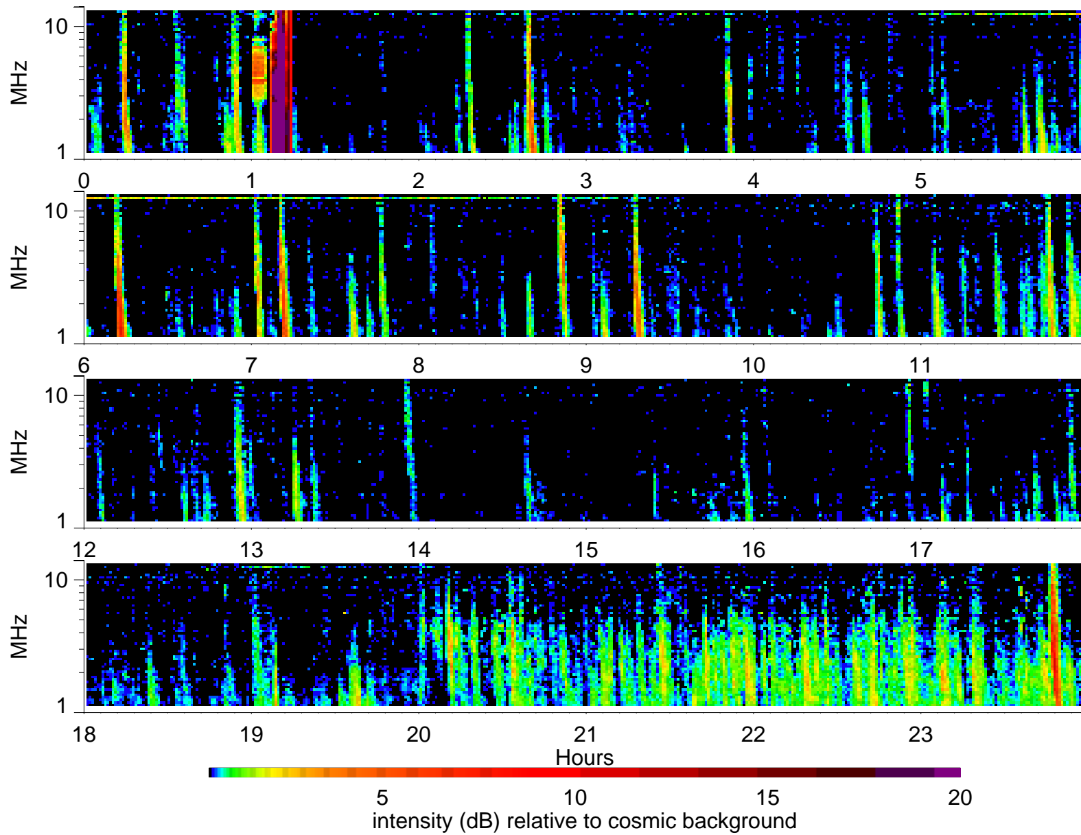
Wind Waves RAD2 receiver: 1998/4/8
