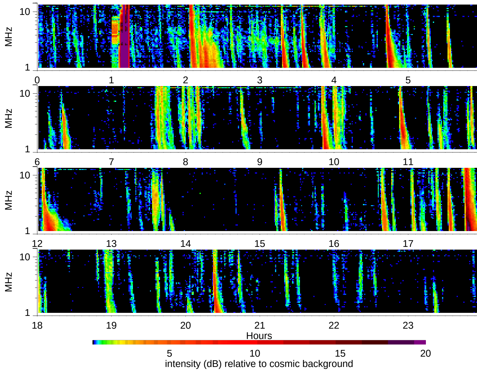
Wind Waves RAD2 receiver: 1998/4/10
