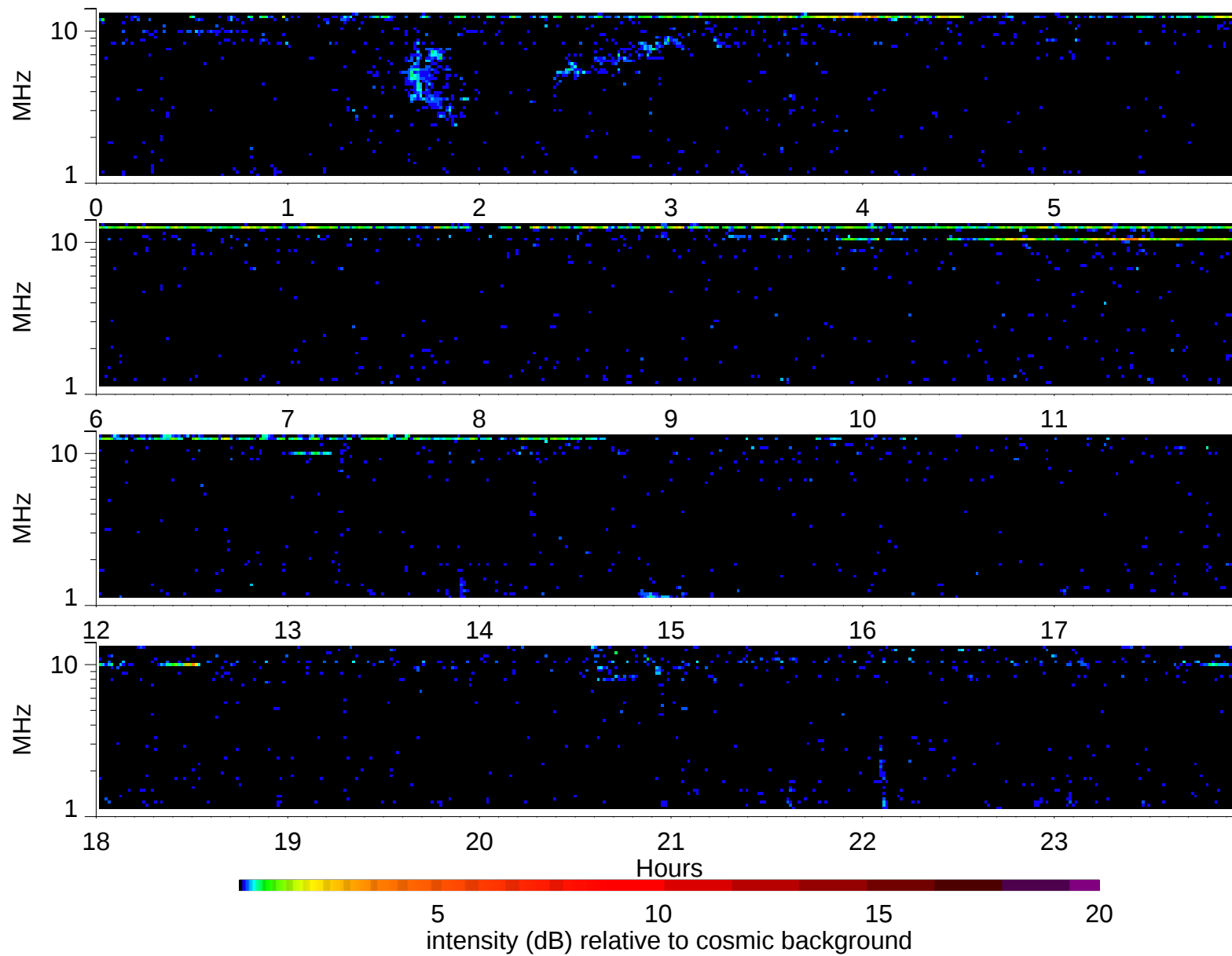
Wind Waves RAD2 receiver: 1998/4/19
