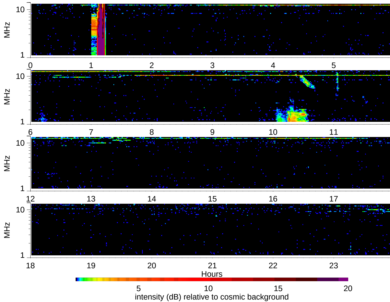
Wind Waves RAD2 receiver: 1998/4/20
