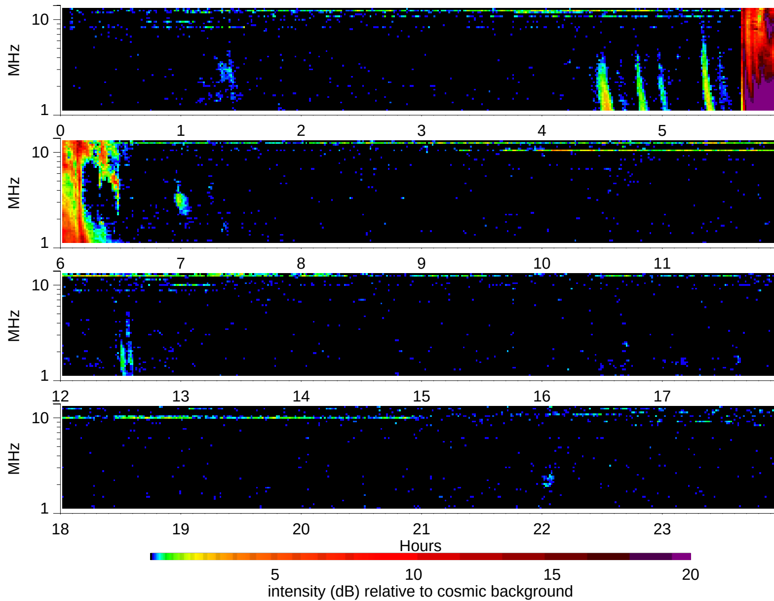
Wind Waves RAD2 receiver: 1998/4/23
