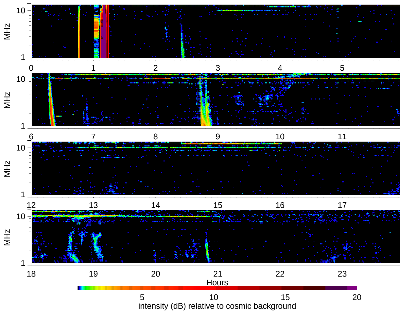
Wind Waves RAD2 receiver: 1998/4/24
