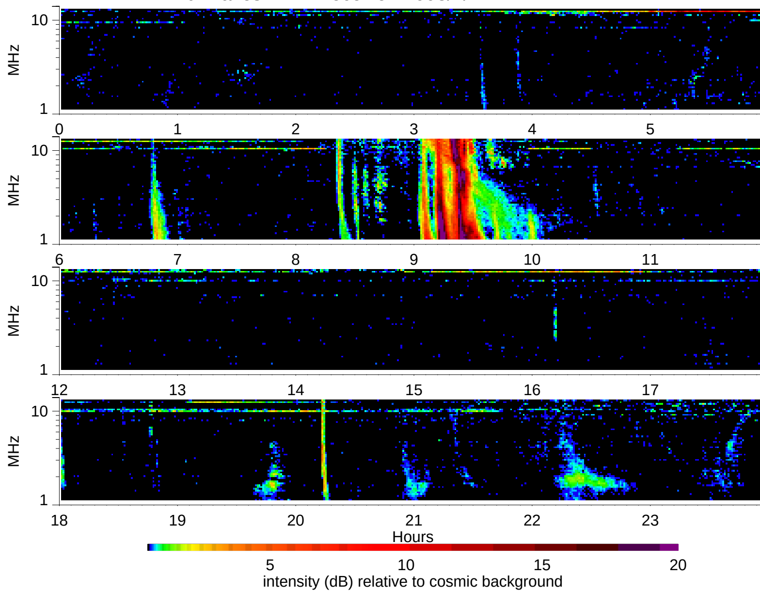
Wind Waves RAD2 receiver: 1998/4/27
