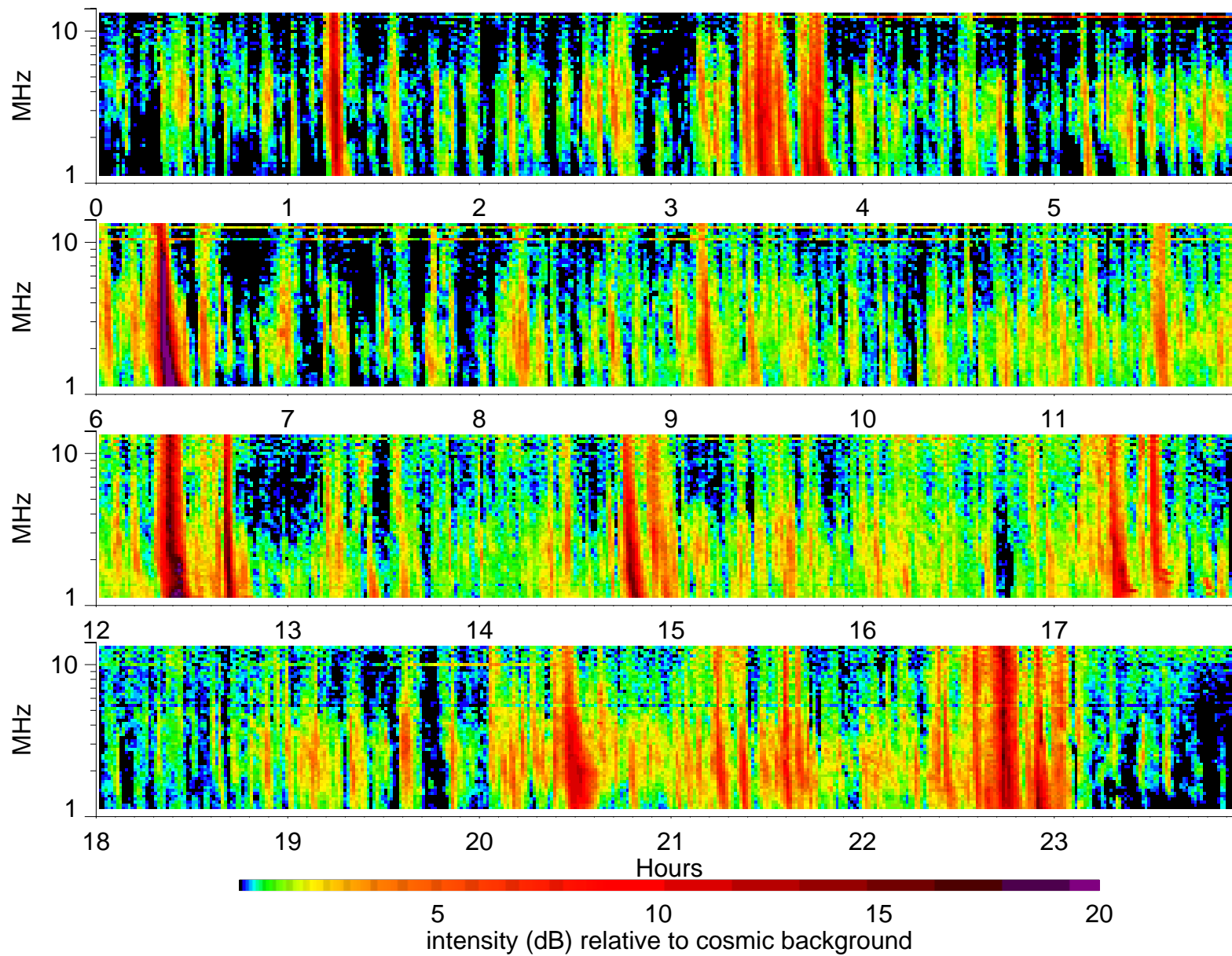
Wind Waves RAD2 receiver: 1998/5/1
