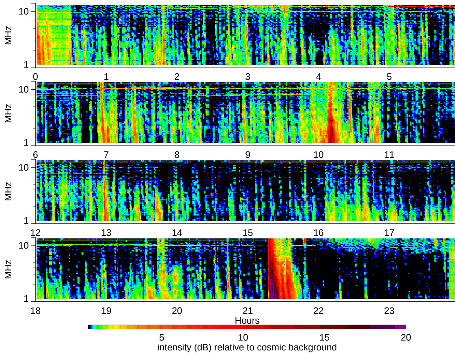
Wind Waves RAD2 receiver: 1998/5/3
