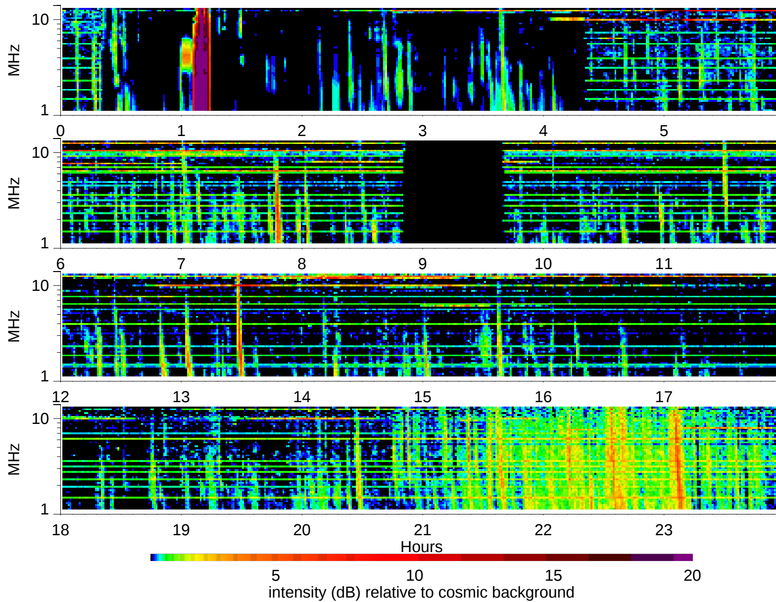
Wind Waves RAD2 receiver: 1998/5/4
