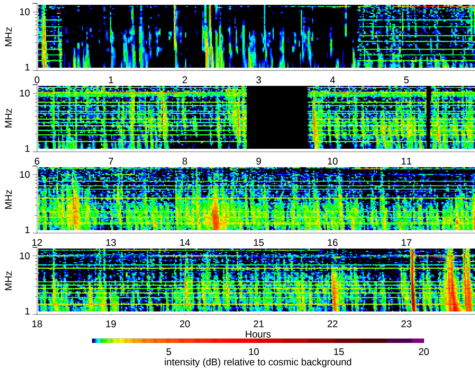
Wind Waves RAD2 receiver: 1998/5/5
