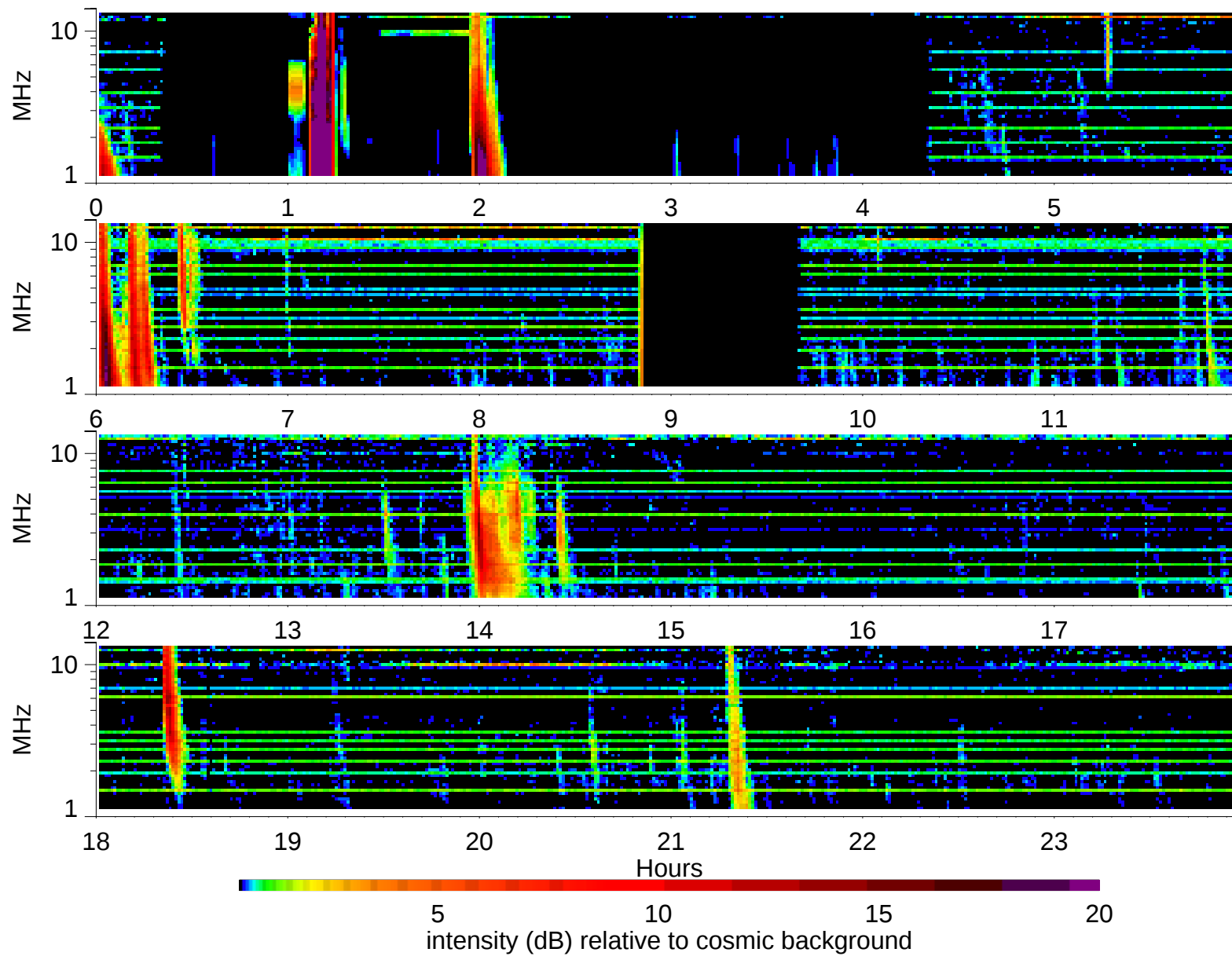
Wind Waves RAD2 receiver: 1998/5/8
