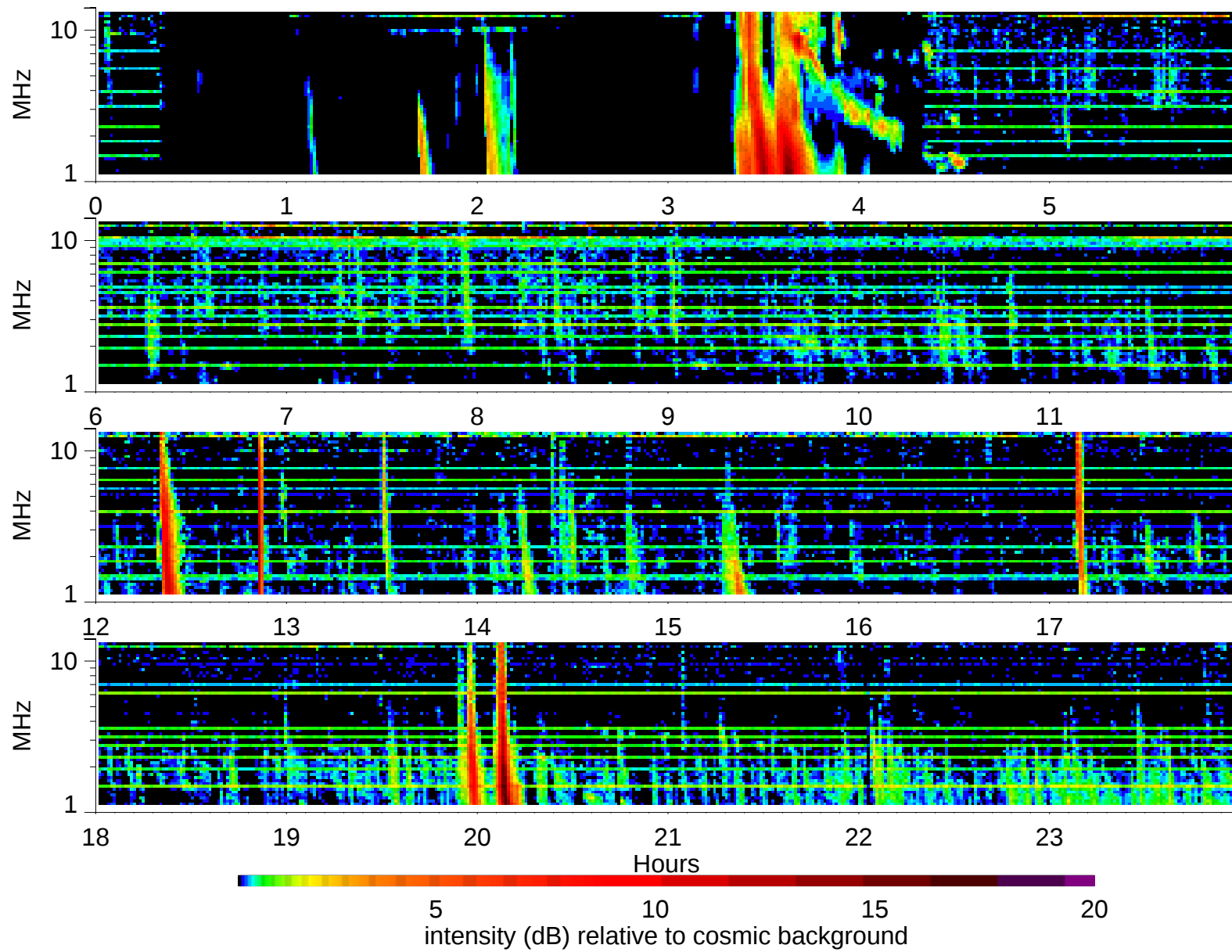
Wind Waves RAD2 receiver: 1998/5/9
