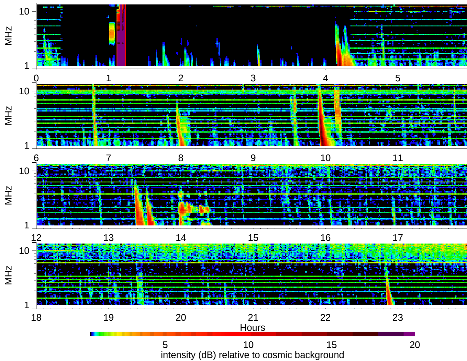
Wind Waves RAD2 receiver: 1998/5/10
