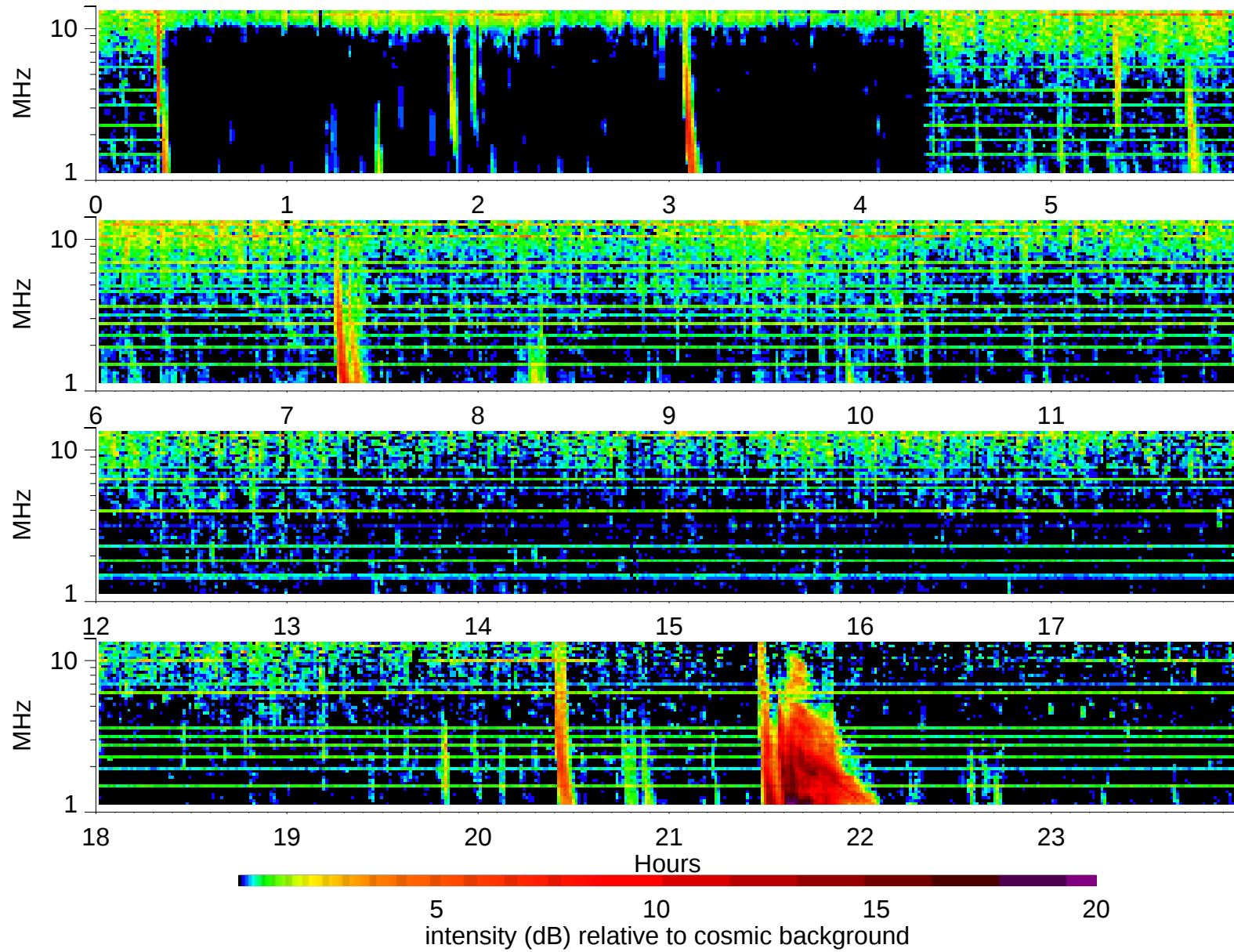
Wind Waves RAD2 receiver: 1998/5/11
