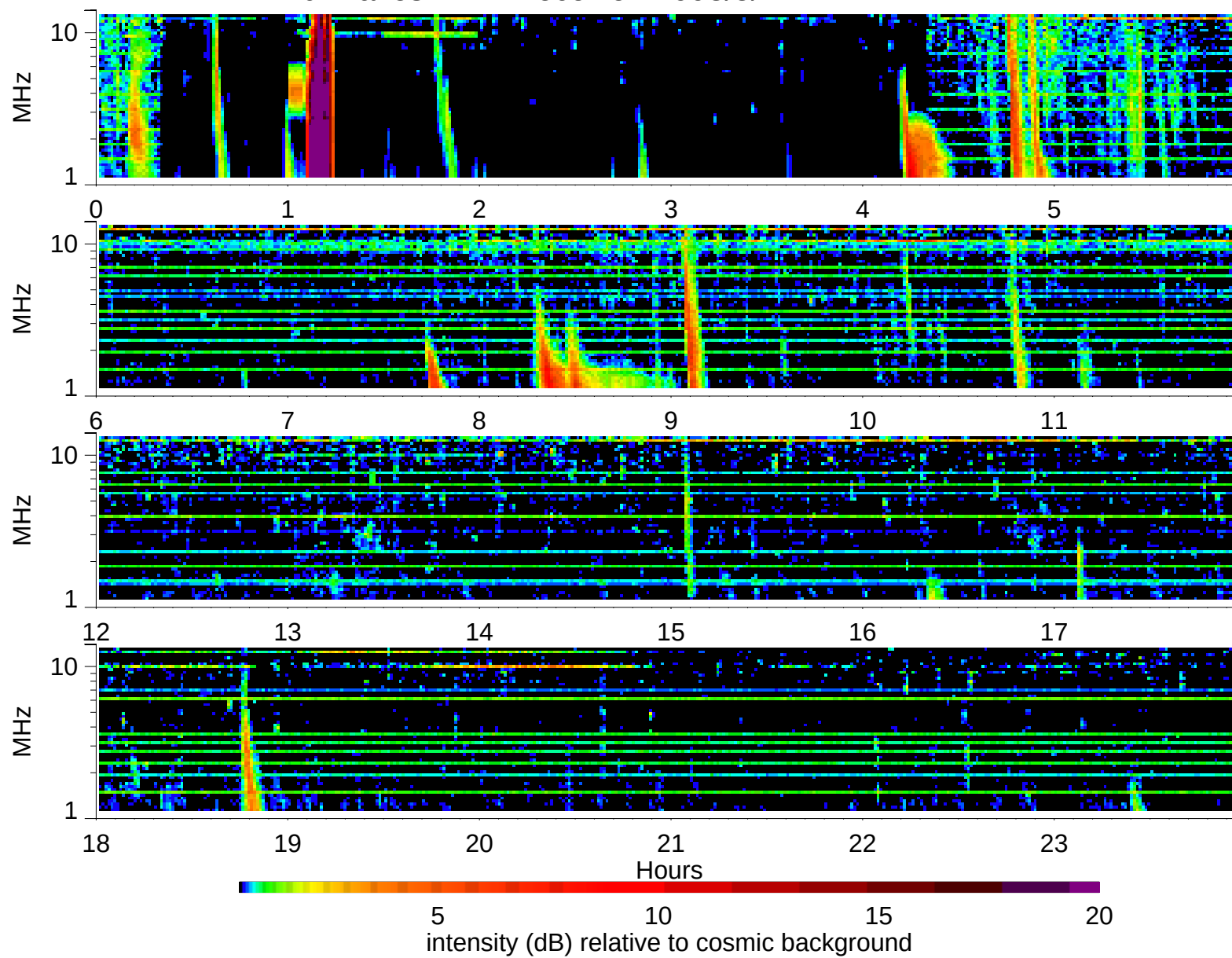
Wind Waves RAD2 receiver: 1998/5/12
