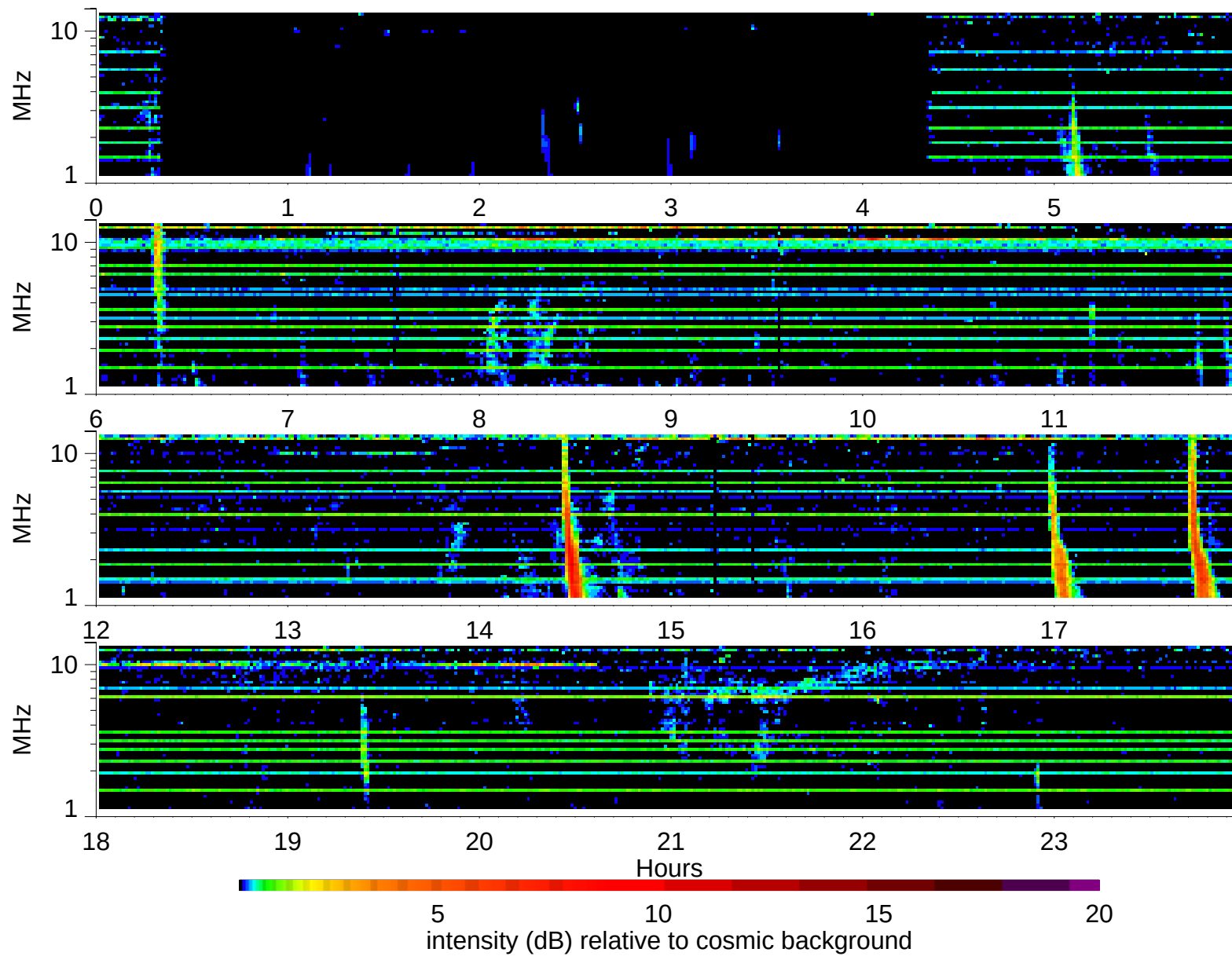
Wind Waves RAD2 receiver: 1998/5/13
