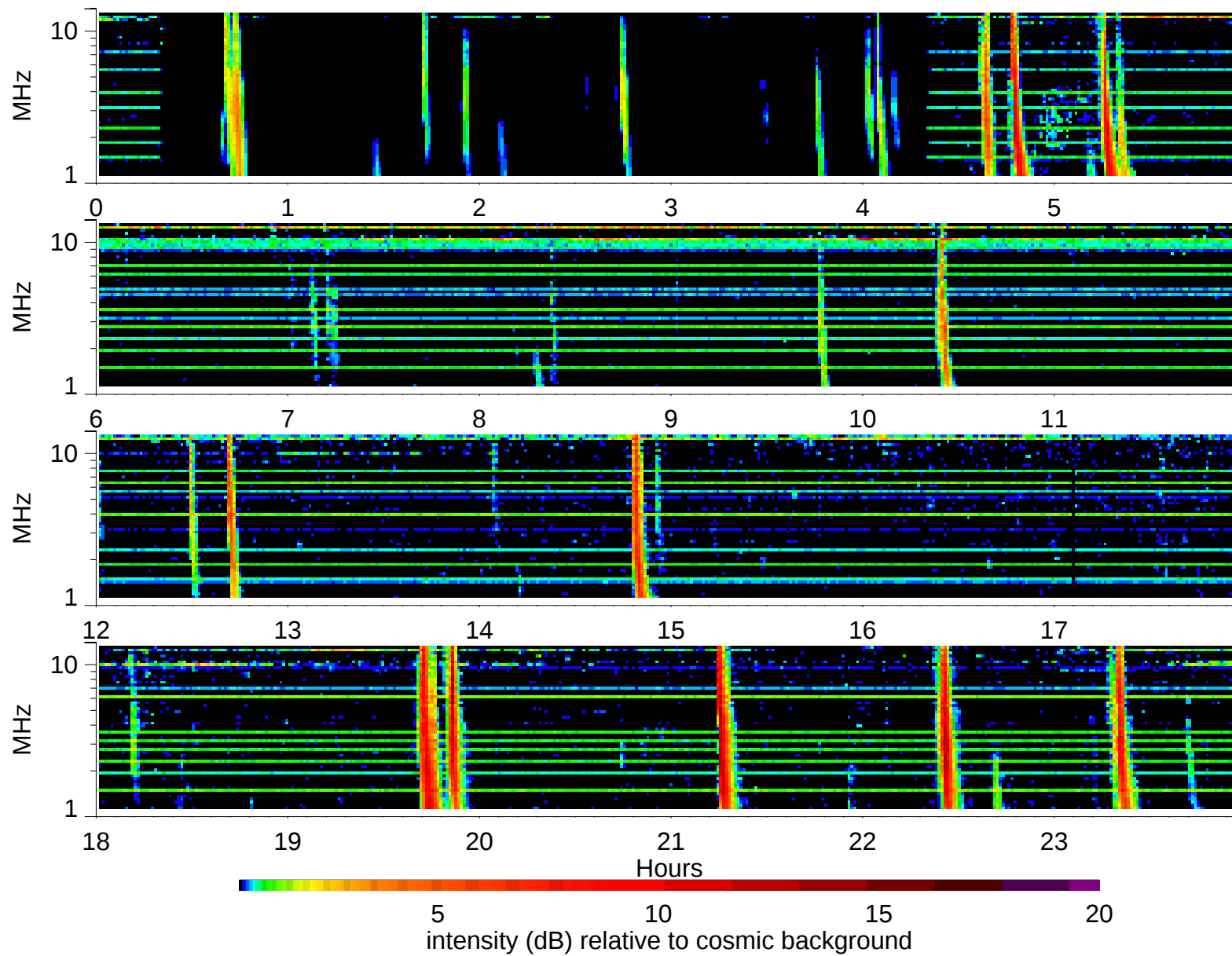
Wind Waves RAD2 receiver: 1998/5/15
