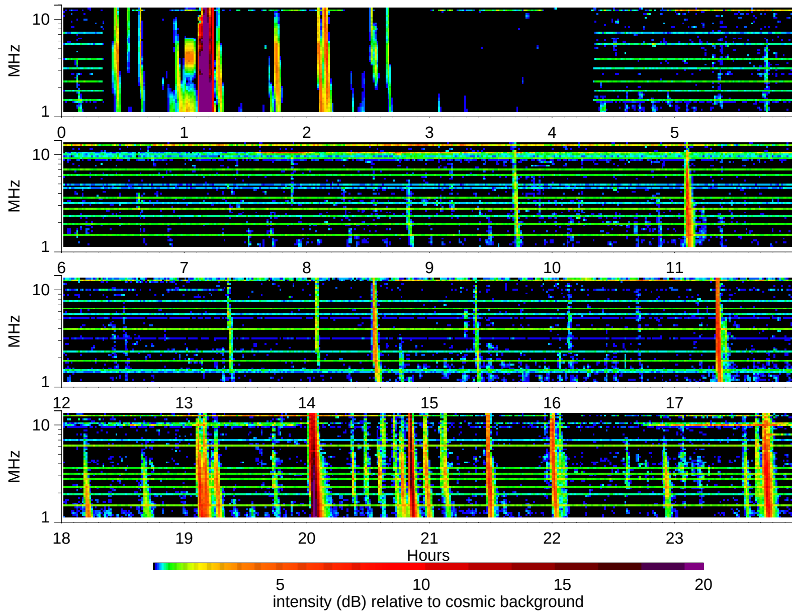
Wind Waves RAD2 receiver: 1998/5/16
