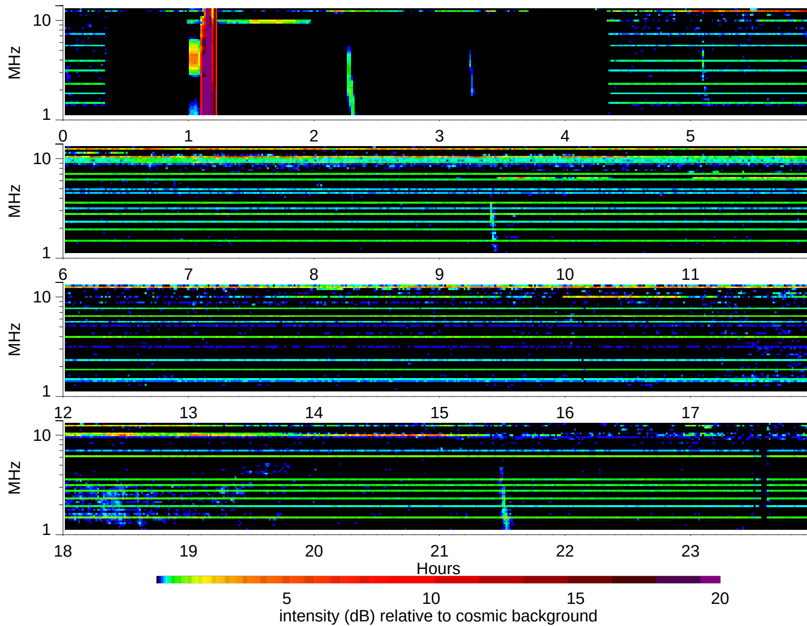
Wind Waves RAD2 receiver: 1998/5/22
