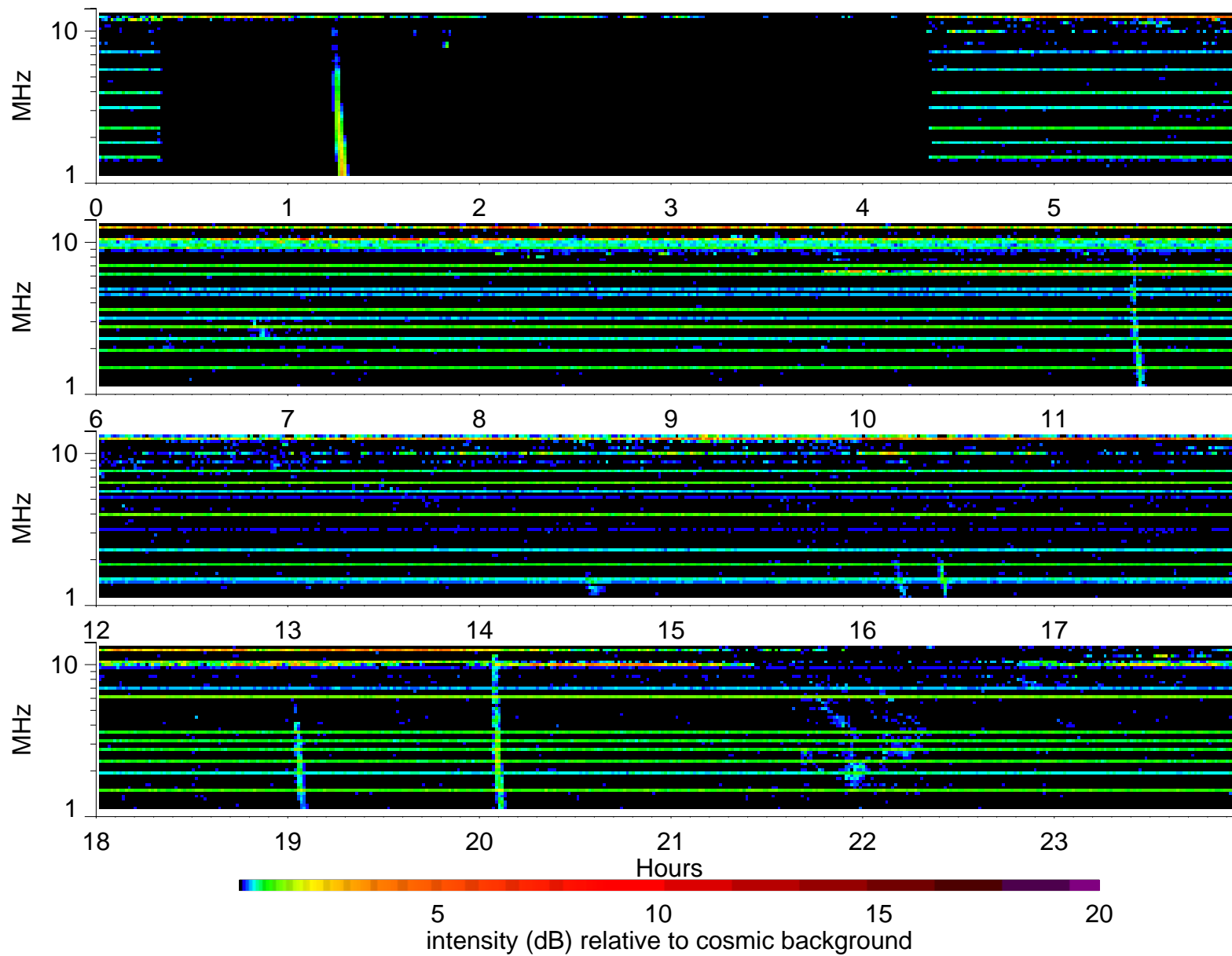
Wind Waves RAD2 receiver: 1998/5/23
