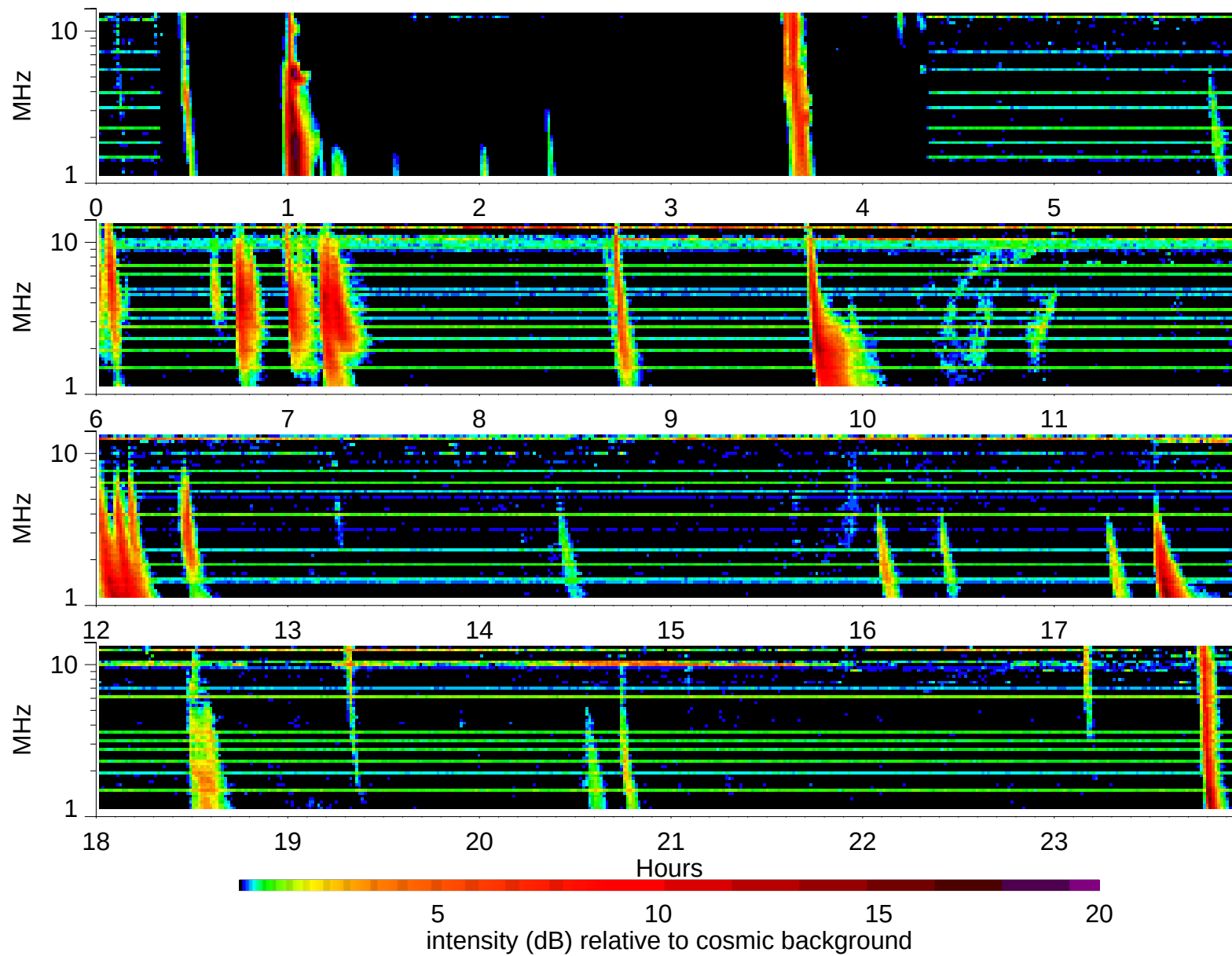
Wind Waves RAD2 receiver: 1998/5/29
