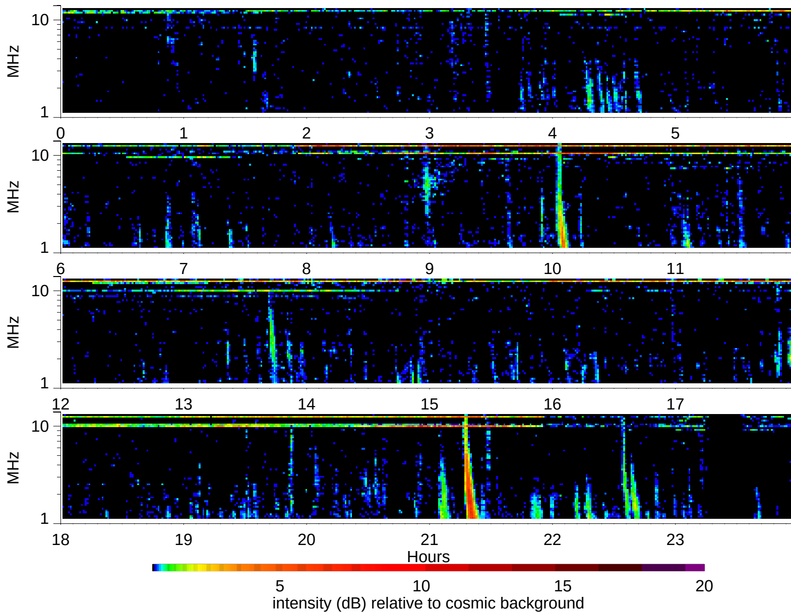
Wind Waves RAD2 receiver: 1998/6/2
