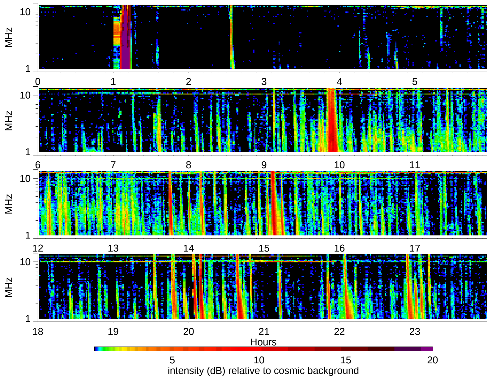
Wind Waves RAD2 receiver: 1998/6/5
