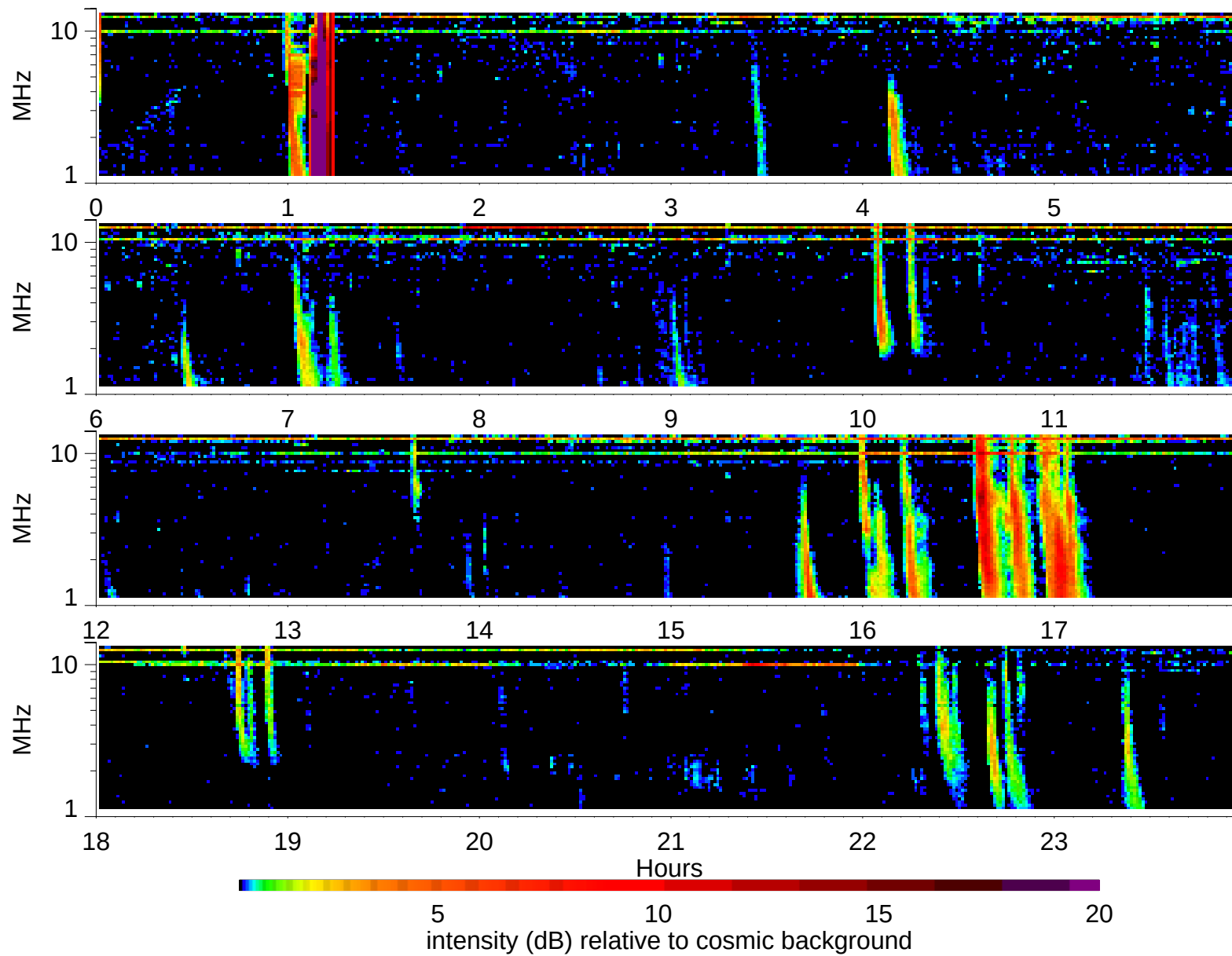
Wind Waves RAD2 receiver: 1998/6/9
