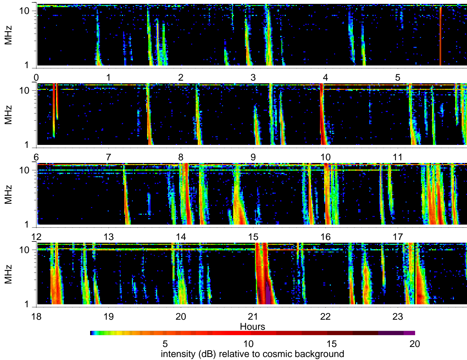
Wind Waves RAD2 receiver: 1998/6/12
