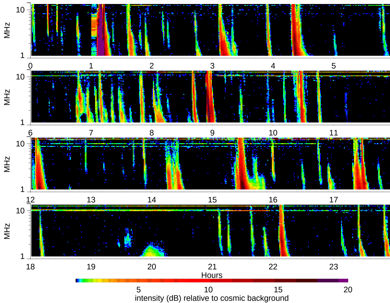
Wind Waves RAD2 receiver: 1998/6/13
