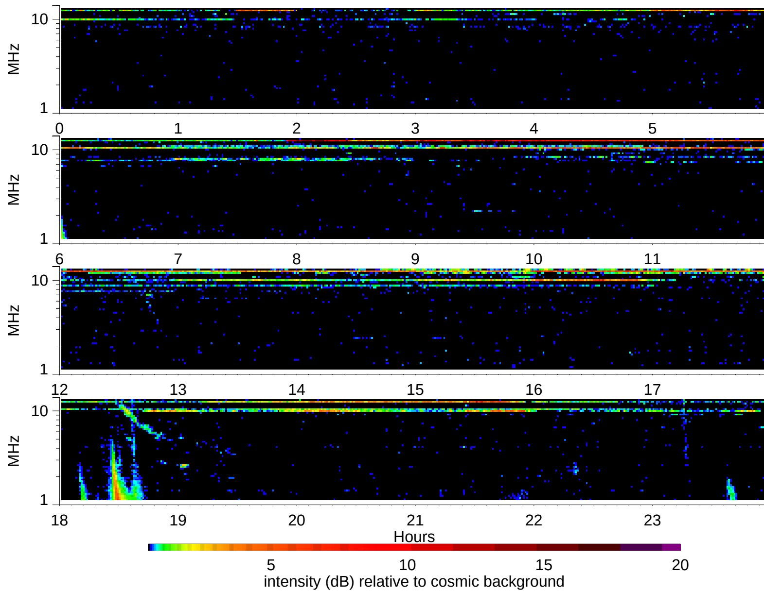
Wind Waves RAD2 receiver: 1998/6/16
