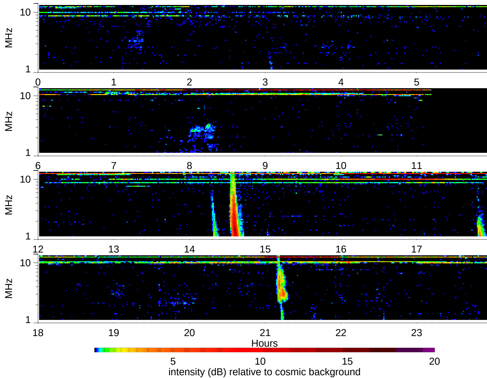
Wind Waves RAD2 receiver: 1998/6/20
